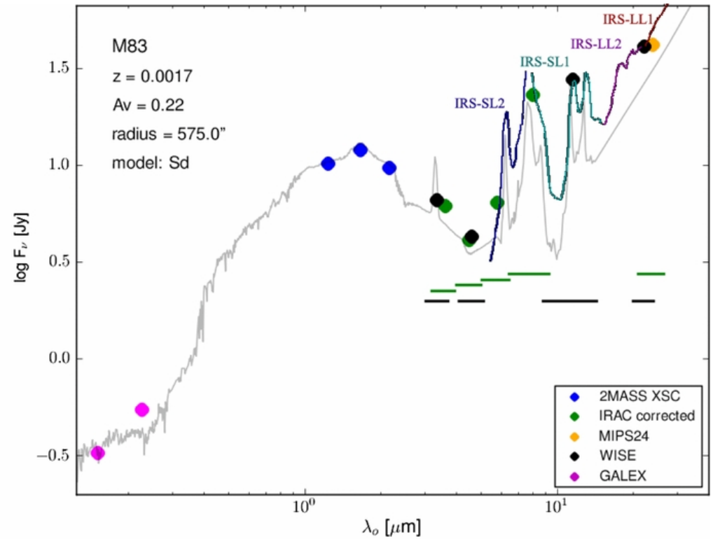
Figure 8. from Extending the Nearby Galaxy Heritage with WISE: First Results from the WISE Enhanced Resolution Galaxy Atlas Jarrett et al. 2013 AJ 145 6 doi:10.1088/0004-6256/145/1/6 https://dx.doi.org/10.1088/0004-6256/145/1/6 © 2013. The American Astronomical Society. All rights reserved.
