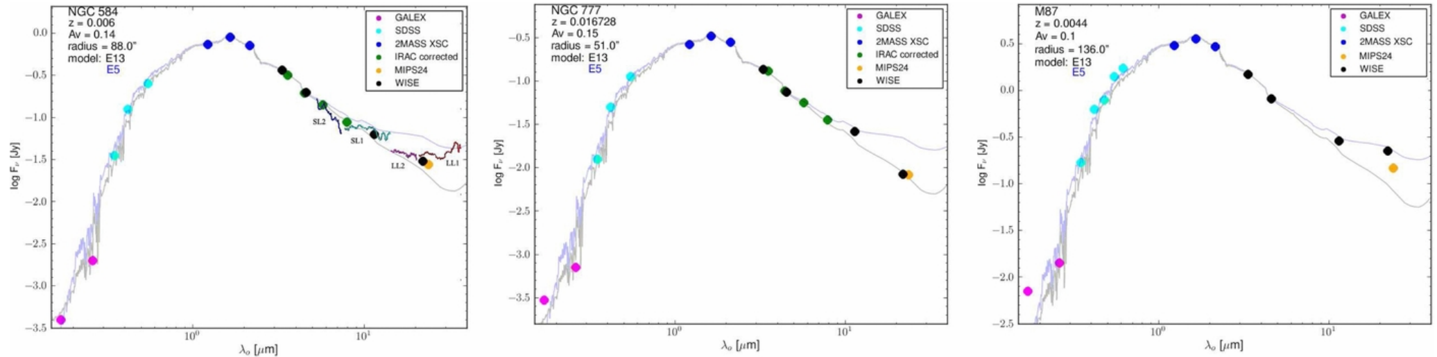
Figure 3. from Extending the Nearby Galaxy Heritage with WISE: First Results from the WISE Enhanced Resolution Galaxy Atlas Jarrett et al. 2013 AJ 145 6 doi:10.1088/0004-6256/145/1/6 https://dx.doi.org/10.1088/0004-6256/145/1/6 © 2013. The American Astronomical Society. All rights reserved.
