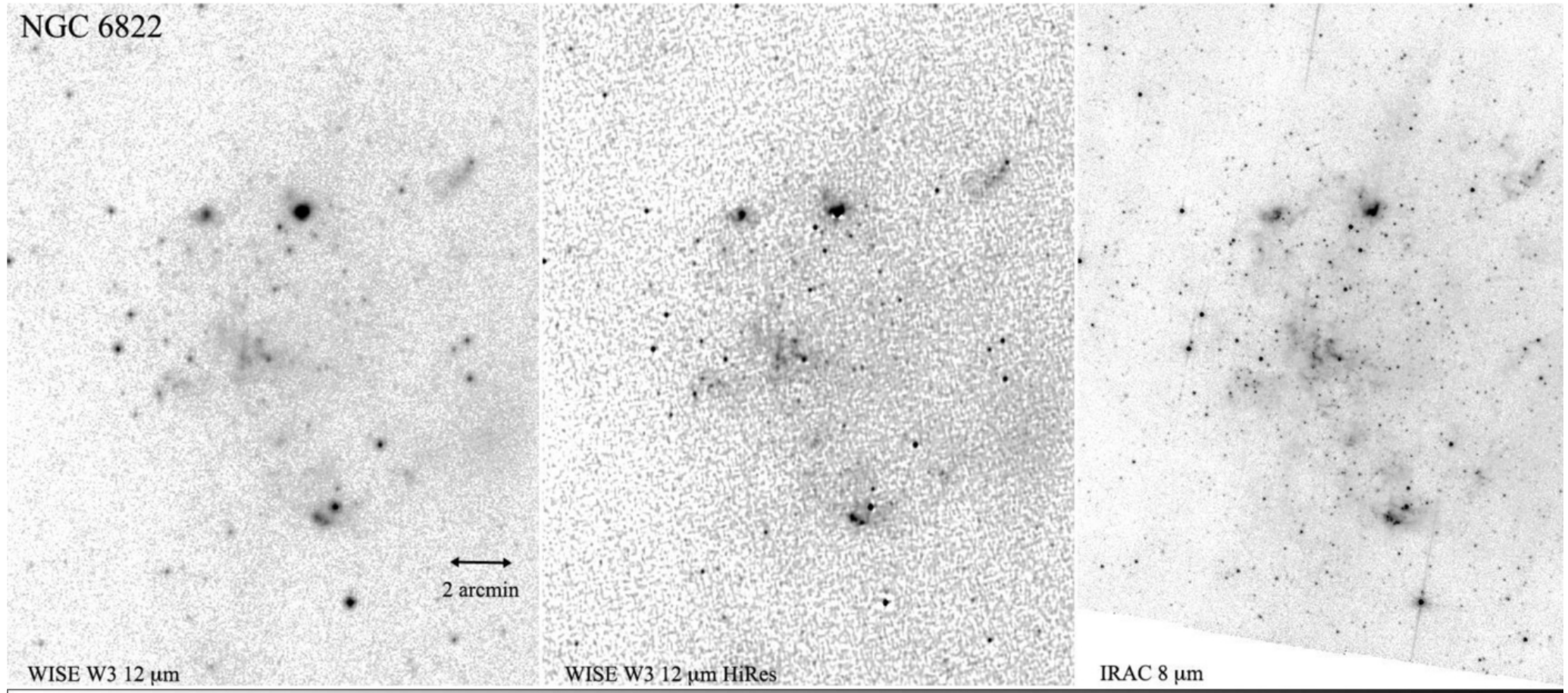
Figure 24. from Extending the Nearby Galaxy Heritage with WISE: First Results from the WISE Enhanced Resolution Galaxy Atlas Jarrett et al. 2013 AJ 145 6 doi:10.1088/0004-6256/145/1/6 https://dx.doi.org/10.1088/0004-6256/145/1/6 © 2013. The American Astronomical Society. All rights reserved.
