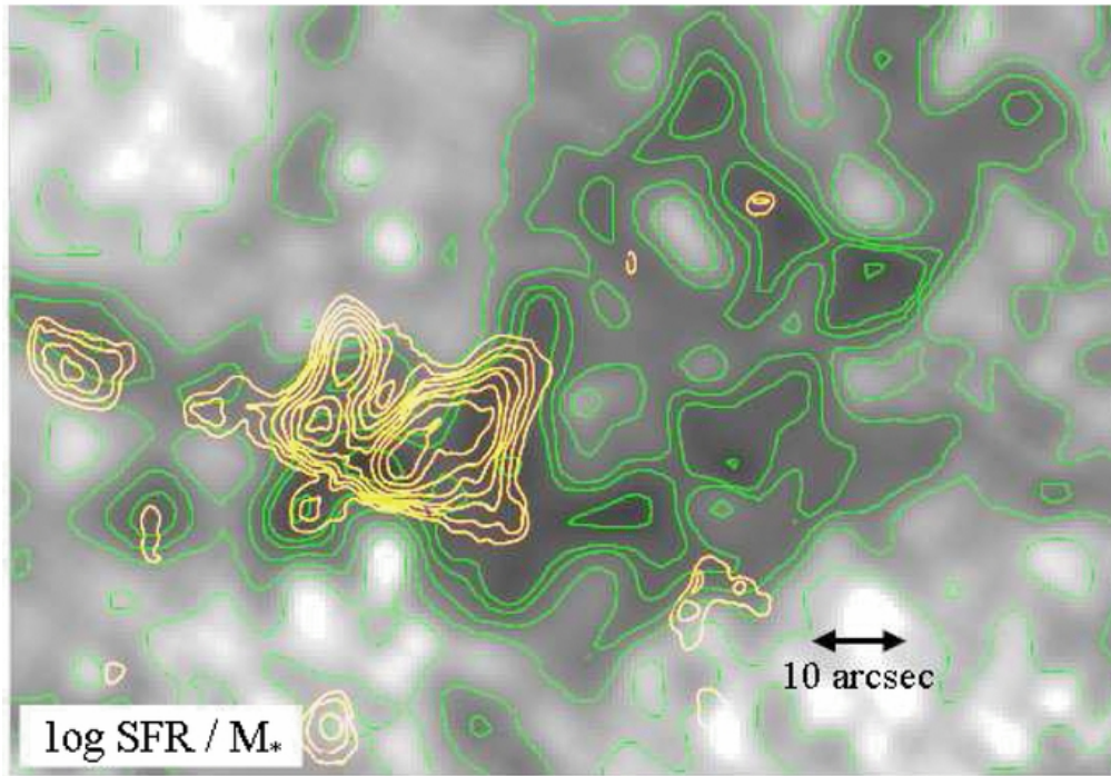
Figure 20. from Extending the Nearby Galaxy Heritage with WISE: First Results from the WISE Enhanced Resolution Galaxy Atlas Jarrett et al. 2013 AJ 145 6 doi:10.1088/0004-6256/145/1/6 https://dx.doi.org/10.1088/0004-6256/145/1/6 © 2013. The American Astronomical Society. All rights reserved.
