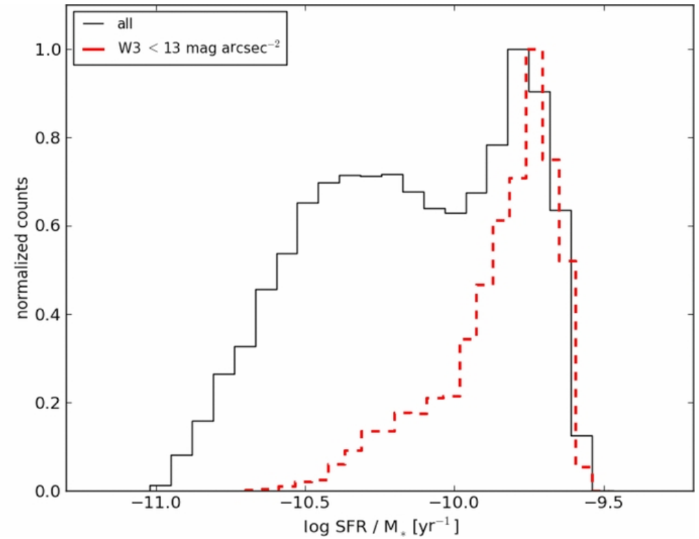
Figure 20. from Extending the Nearby Galaxy Heritage with WISE: First Results from the WISE Enhanced Resolution Galaxy Atlas Jarrett et al. 2013 AJ 145 6 doi:10.1088/0004-6256/145/1/6 https://dx.doi.org/10.1088/0004-6256/145/1/6 © 2013. The American Astronomical Society. All rights reserved.
