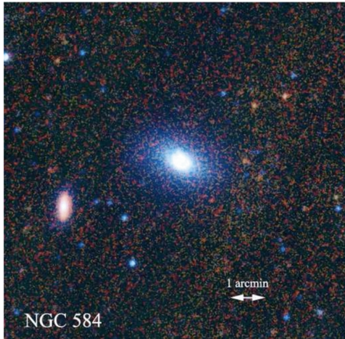
Figure 2. from Extending the Nearby Galaxy Heritage with WISE: First Results from the WISE Enhanced Resolution Galaxy Atlas Jarrett et al. 2013 AJ 145 6 doi:10.1088/0004-6256/145/1/6 https://dx.doi.org/10.1088/0004-6256/145/1/6 © 2013. The American Astronomical Society. All rights reserved.
