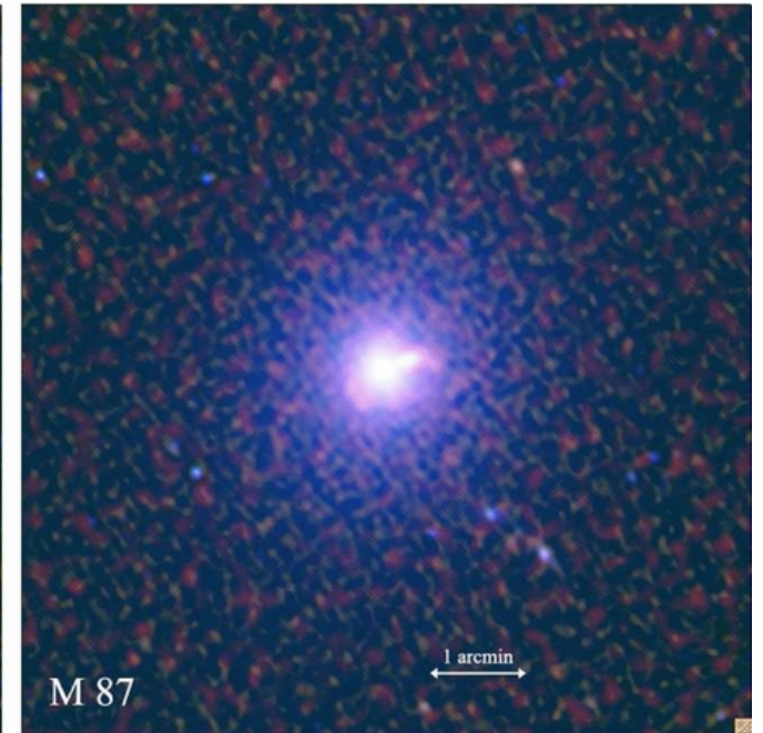
Figure 2. from Extending the Nearby Galaxy Heritage with WISE: First Results from the WISE Enhanced Resolution Galaxy Atlas Jarrett et al. 2013 AJ 145 6 doi:10.1088/0004-6256/145/1/6 https://dx.doi.org/10.1088/0004-6256/145/1/6 © 2013. The American Astronomical Society. All rights reserved.
