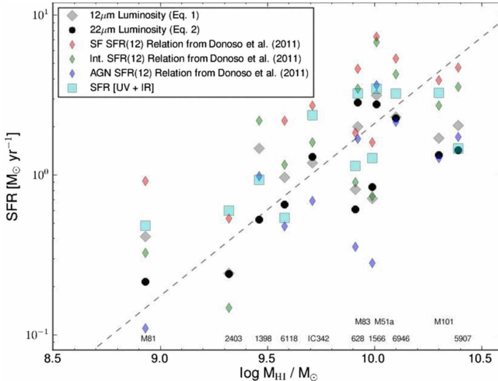
Figure 16. from Extending the Nearby Galaxy Heritage with WISE: First Results from the WISE Enhanced Resolution Galaxy Atlas Jarrett et al. 2013 AJ 145 6 doi:10.1088/0004-6256/145/1/6 https://dx.doi.org/10.1088/0004-6256/145/1/6 © 2013. The American Astronomical Society. All rights reserved.
