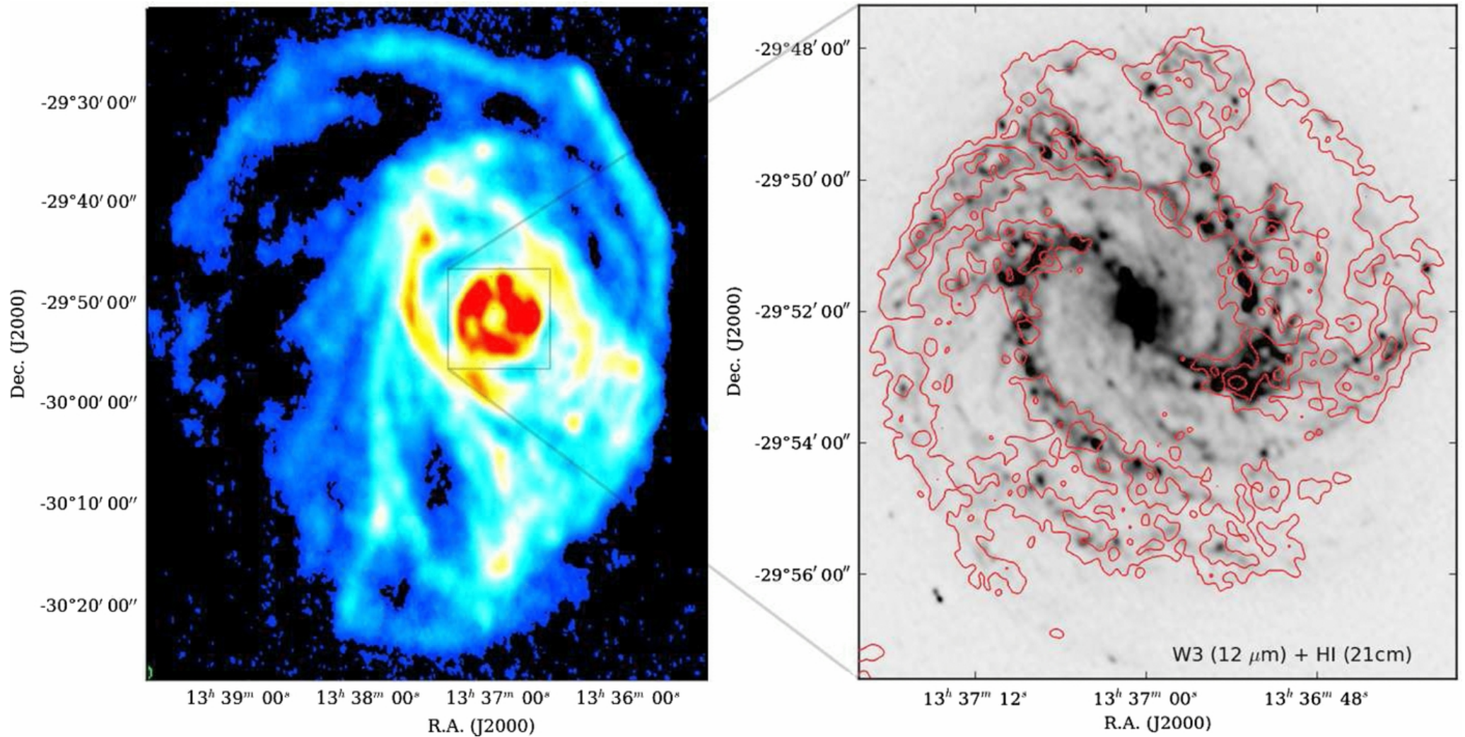
Figure 12. from Extending the Nearby Galaxy Heritage with WISE: First Results from the WISE Enhanced Resolution Galaxy Atlas Jarrett et al. 2013 AJ 145 6 doi:10.1088/0004-6256/145/1/6 https://dx.doi.org/10.1088/0004-6256/145/1/6 © 2013. The American Astronomical Society. All rights reserved.
