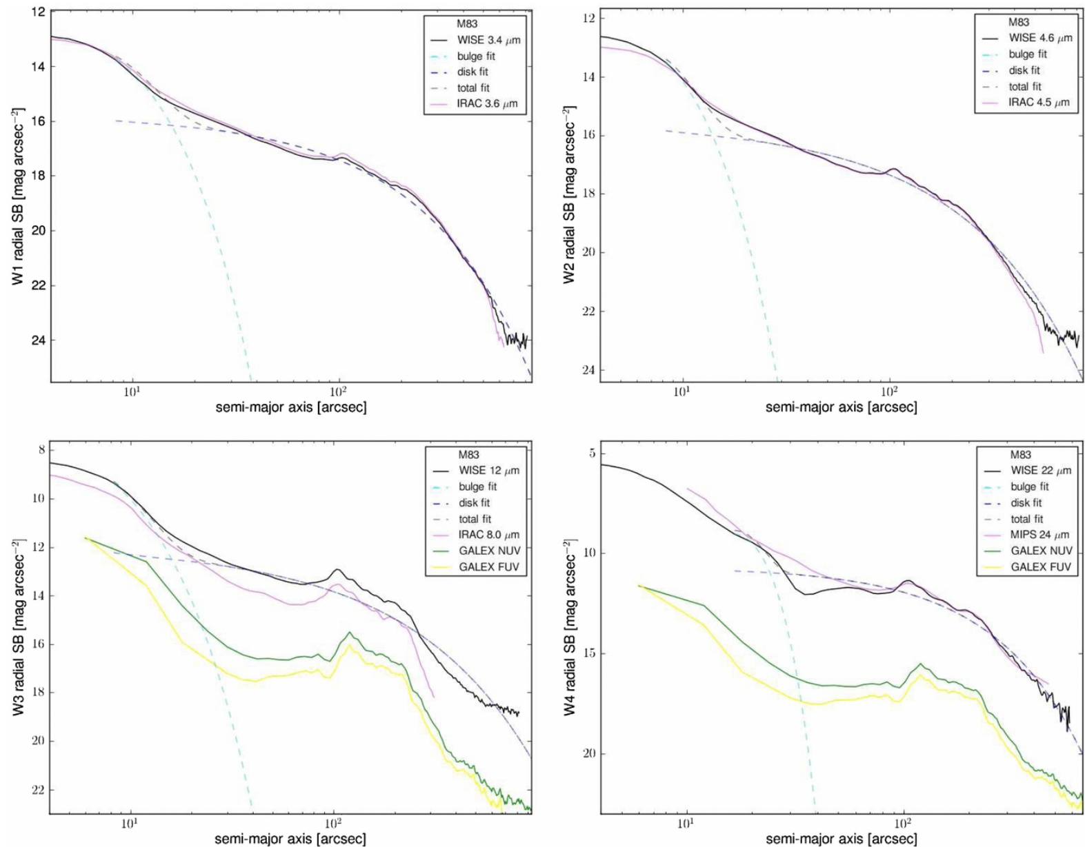
Figure 11. from Extending the Nearby Galaxy Heritage with WISE: First Results from the WISE Enhanced Resolution Galaxy Atlas Jarrett et al. 2013 AJ 145 6 doi:10.1088/0004-6256/145/1/6 https://dx.doi.org/10.1088/0004-6256/145/1/6
