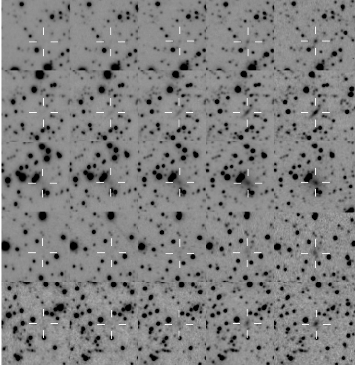
Figure 6. from Galaxies behind the Galactic Plane: First Results and Perspectives from the VVV Survey Amôres et al. 2012 AJ 144 127 doi:10.1088/0004-6256/144/5/127 https://dx.doi.org/10.1088/0004-6256/144/5/127 © 2012. The American Astronomical Society. All rights reserved.
