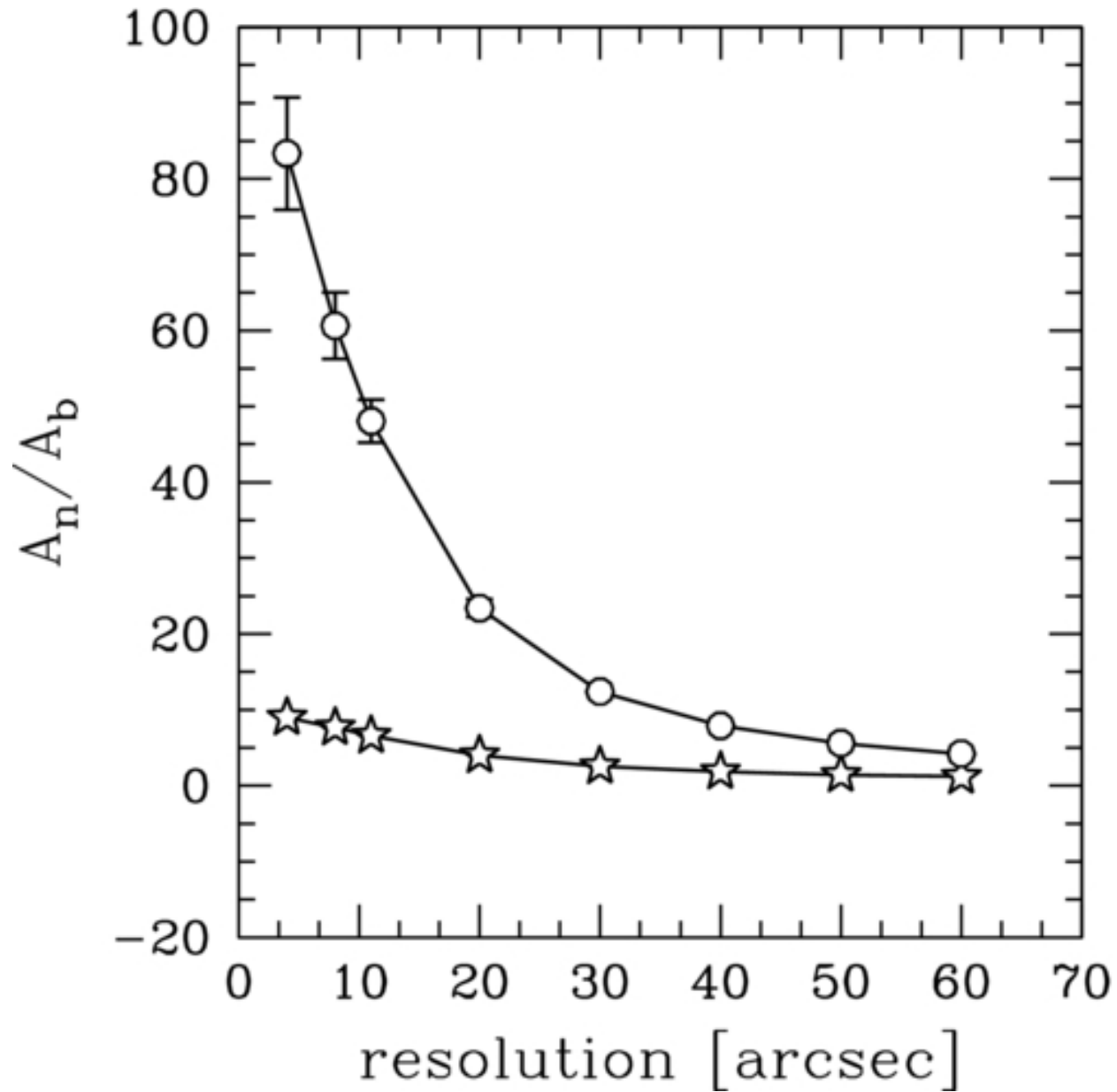
Figure 6. from The Shapes of the H I Velocity Profiles of the THINGS Galaxies Ianjamasimanana et al. 2012 AJ 144 96 doi:10.1088/0004-6256/144/4/96 https://dx.doi.org/10.1088/0004-6256/144/4/96 © 2012. The American Astronomical Society. All rights reserved.
