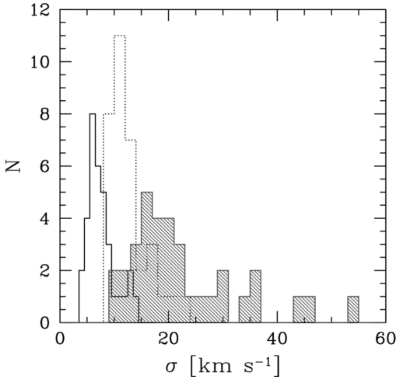
Figure 3. from The Shapes of the H I Velocity Profiles of the THINGS Galaxies Ianjamasimanana et al. 2012 AJ 144 96 doi:10.1088/0004-6256/144/4/96 https://dx.doi.org/10.1088/0004-6256/144/4/96 © 2012. The American Astronomical Society. All rights reserved.
