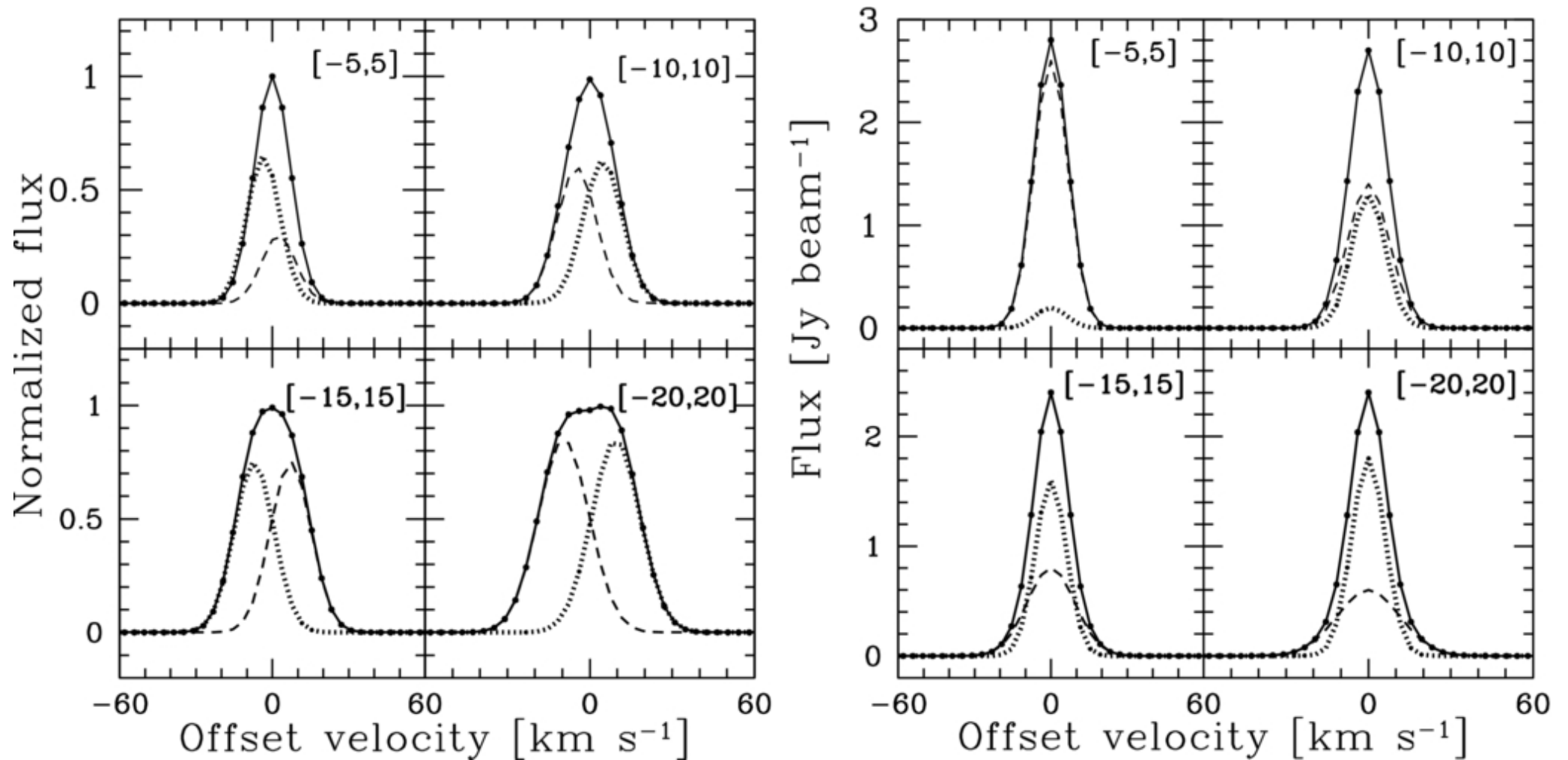
Figure 27. from The Shapes of the H I Velocity Profiles of the THINGS Galaxies Ianjamasimanana et al. 2012 AJ 144 96 doi:10.1088/0004-6256/144/4/96 https://dx.doi.org/10.1088/0004-6256/144/4/96 © 2012. The American Astronomical Society. All rights reserved.
