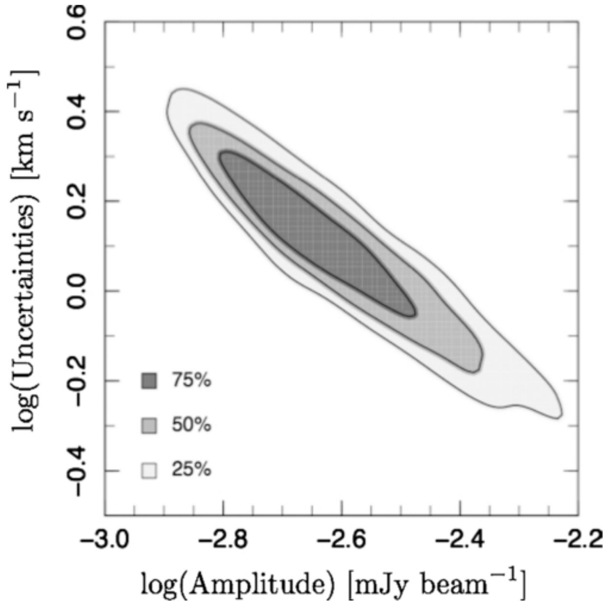
Figure 26. from The Shapes of the H I Velocity Profiles of the THINGS Galaxies Ianjamasimanana et al. 2012 AJ 144 96 doi:10.1088/0004-6256/144/4/96 https://dx.doi.org/10.1088/0004-6256/144/4/96 © 2012. The American Astronomical Society. All rights reserved.
