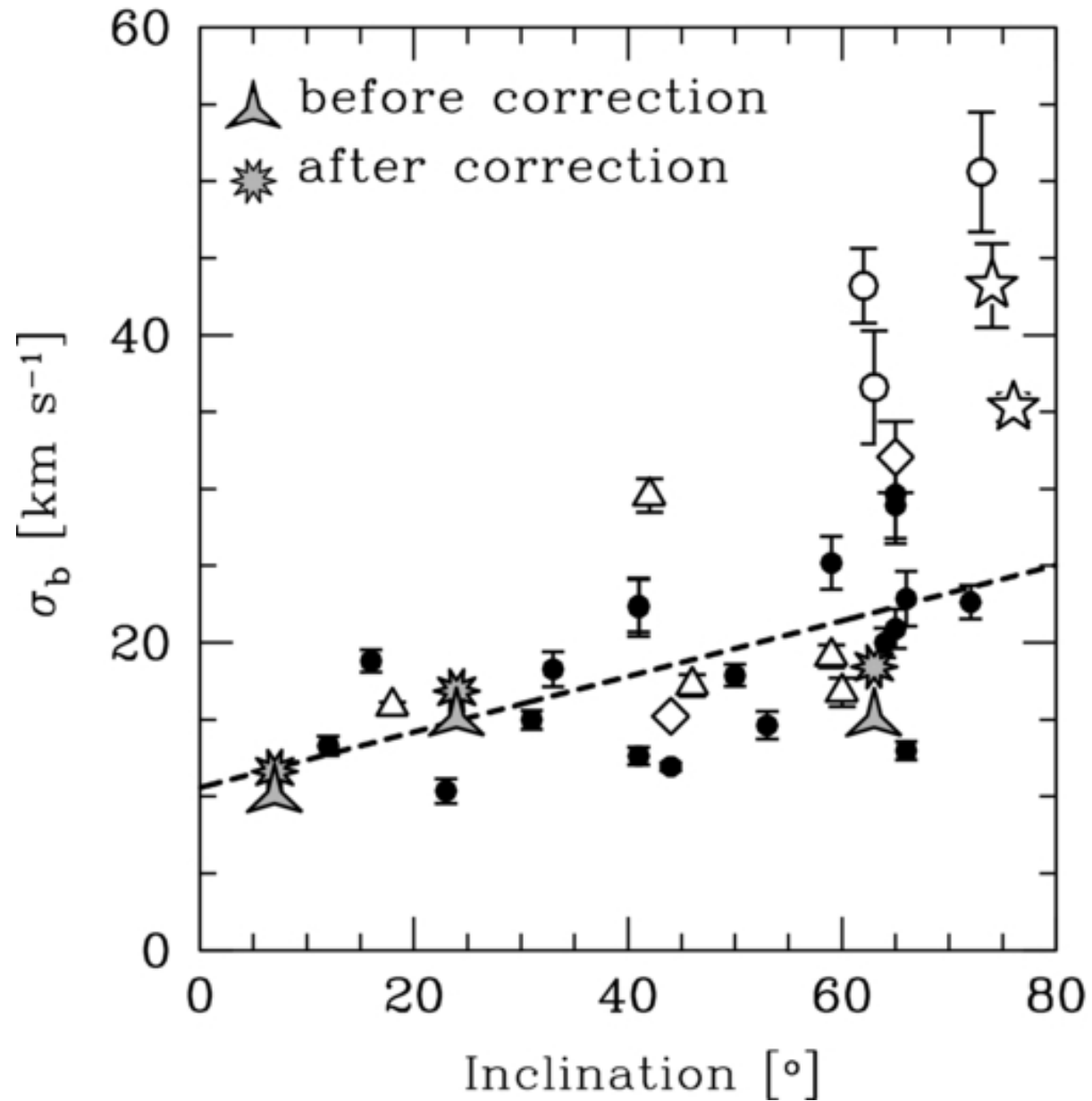
Figure 24. from The Shapes of the H I Velocity Profiles of the THINGS Galaxies Ianjamasimanana et al. 2012 AJ 144 96 doi:10.1088/0004-6256/144/4/96 https://dx.doi.org/10.1088/0004-6256/144/4/96 © 2012. The American Astronomical Society. All rights reserved.
