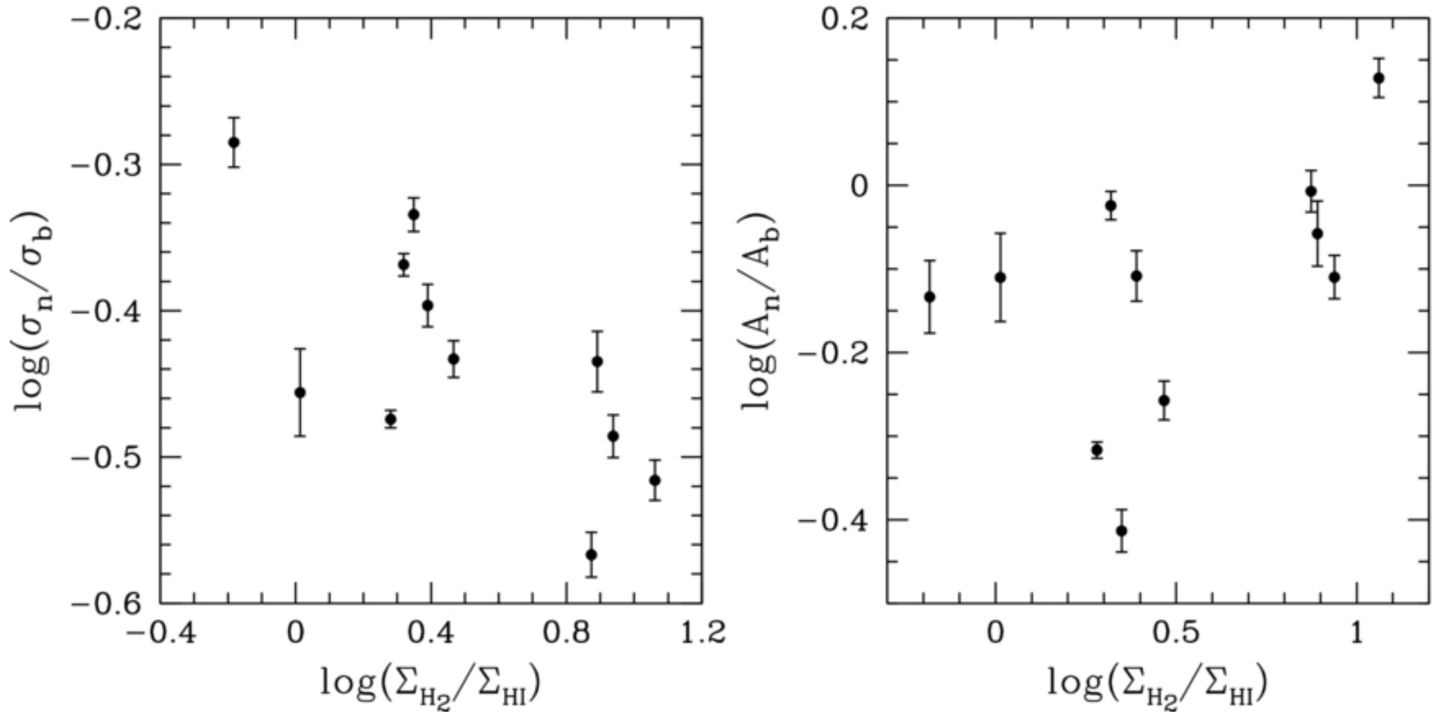
Figure 23. from The Shapes of the H I Velocity Profiles of the THINGS Galaxies Ianjamasimanana et al. 2012 AJ 144 96 doi:10.1088/0004-6256/144/4/96 https://dx.doi.org/10.1088/0004-6256/144/4/96 © 2012. The American Astronomical Society. All rights reserved.
