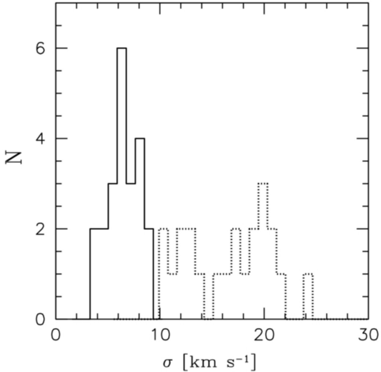
Figure 21. from The Shapes of the H I Velocity Profiles of the THINGS Galaxies Ianjamasimanana et al. 2012 AJ 144 96 doi:10.1088/0004-6256/144/4/96 https://dx.doi.org/10.1088/0004-6256/144/4/96 © 2012. The American Astronomical Society. All rights reserved.
