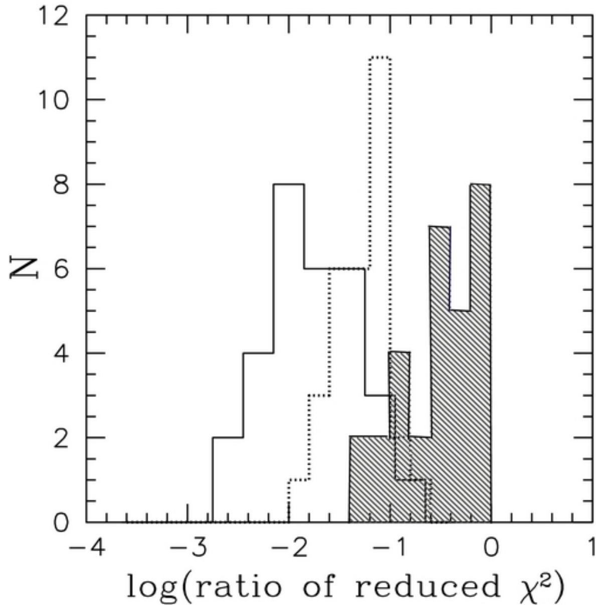
Figure 2. from The Shapes of the H I Velocity Profiles of the THINGS Galaxies Ilanjamasimanana et al. 2012 AJ 144 96 doi:10.1088/0004-6256/144/4/96 https://dx.doi.org/10.1088/0004-6256/144/4/96 © 2012. The American Astronomical Society. All rights reserved.
