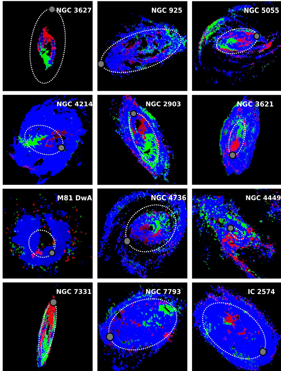
Figure 17. from The Shapes of the H I Velocity Profiles of the THINGS Galaxies Ianjamasimanana et al. 2012 AJ 144 96 doi:10.1088/0004-6256/144/4/96 https://dx.doi.org/10.1088/0004-6256/144/4/96 © 2012. The American Astronomical Society. All rights reserved.
