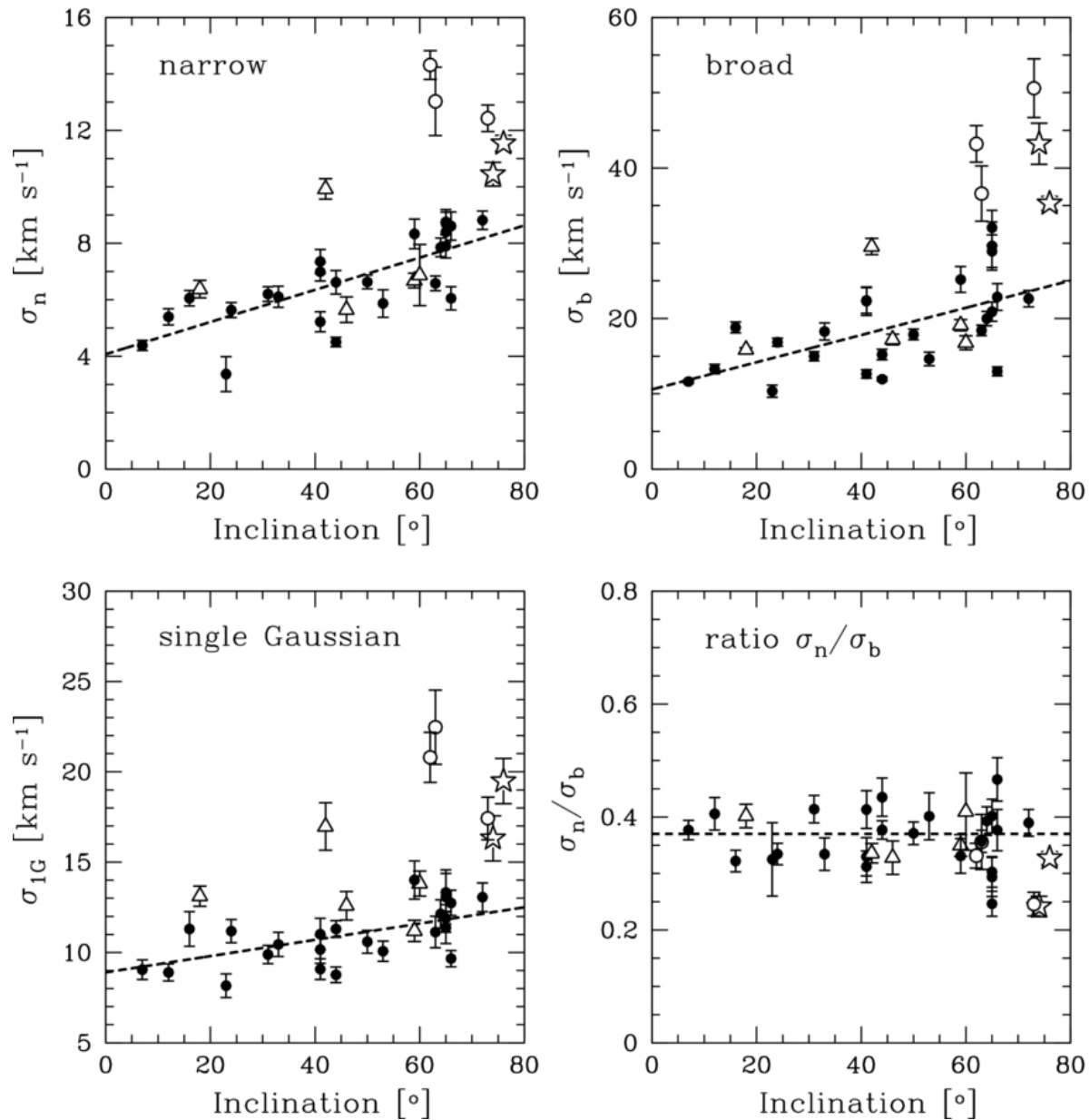
Figure 16. from The Shapes of the H I Velocity Profiles of the THINGS Galaxies Ianjamasimanana et al. 2012 AJ 144 96 doi:10.1088/0004-6256/144/4/96 https://dx.doi.org/10.1088/0004-6256/144/4/96
