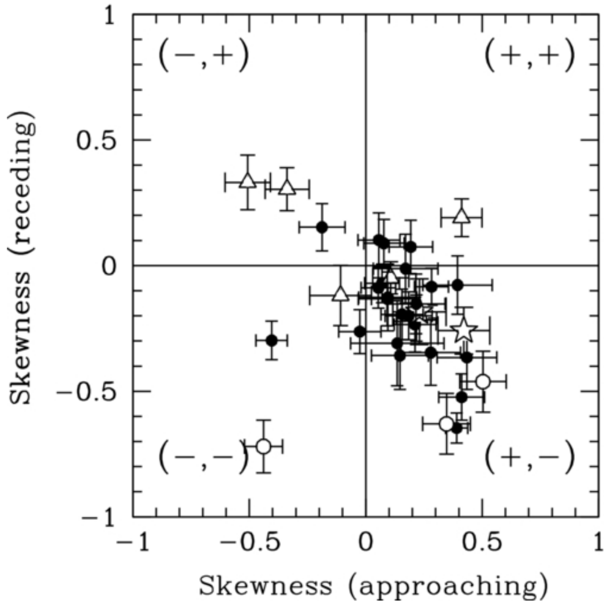
Figure 15. from The Shapes of the H I Velocity Profiles of the THINGS Galaxies Ianjamasimanana et al. 2012 AJ 144 96 doi:10.1088/0004-6256/144/4/96 https://dx.doi.org/10.1088/0004-6256/144/4/96 © 2012. The American Astronomical Society. All rights reserved.
