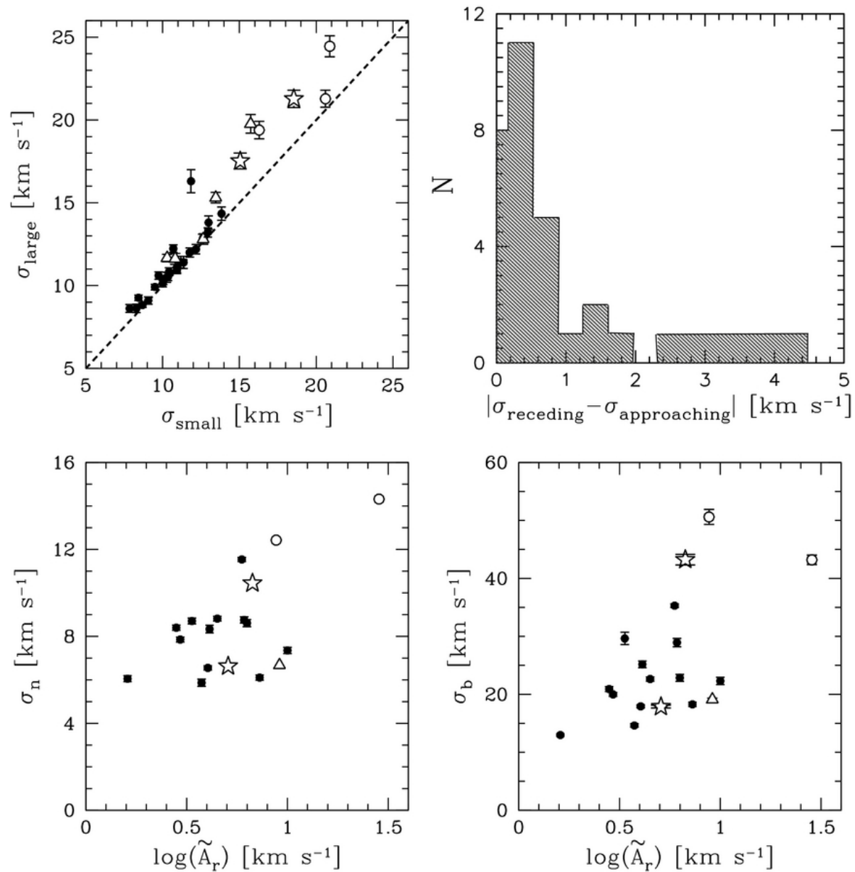
Figure 14. from The Shapes of the H I Velocity Profiles of the THINGS Galaxies Ianjamasimanana et al. 2012 AJ 144 96 doi:10.1088/0004-6256/144/4/96 https://dx.doi.org/10.1088/0004-6256/144/4/96 © 2012. The American Astronomical Society. All rights reserved.
