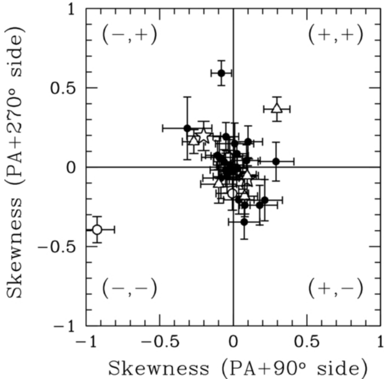
Figure 11. from The Shapes of the H I Velocity Profiles of the THINGS Galaxies Ianjamasimanana et al. 2012 AJ 144 96 doi:10.1088/0004-6256/144/4/96 https://dx.doi.org/10.1088/0004-6256/144/4/96 © 2012. The American Astronomical Society. All rights reserved.
