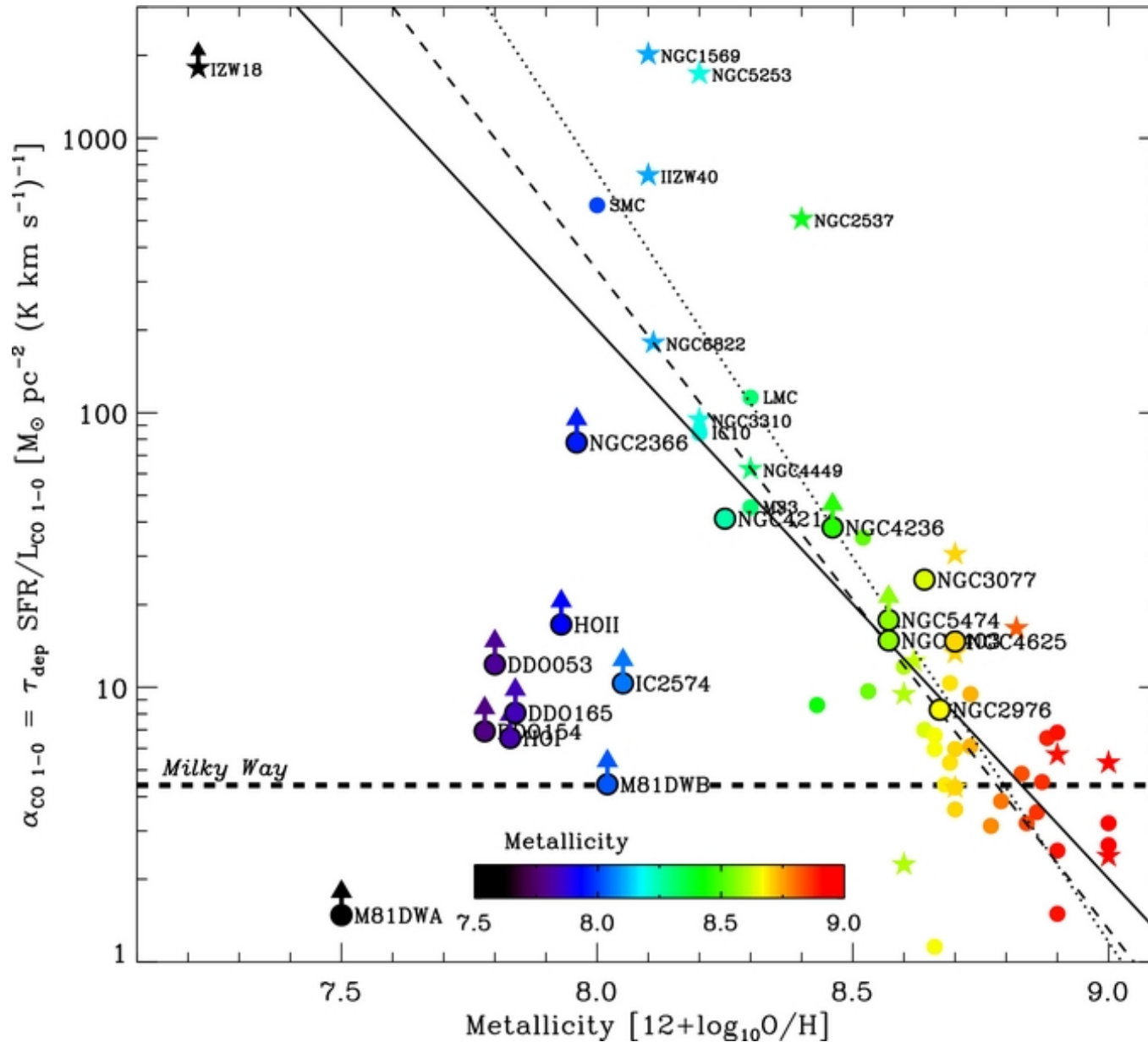
Figure 6. from Low CO Luminosities in Dwarf Galaxies Schrubba et al. 2012 AJ 143 138 doi:10.1088/0004-6256/143/6/138 https://dx.doi.org/10.1088/0004-6256/143/6/138 © 2012. The American Astronomical Society. All rights reserved.
