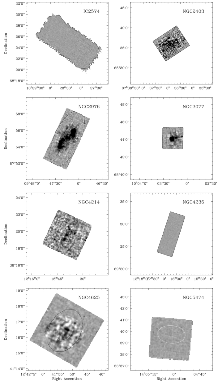
Figure 2. from Low CO Luminosities in Dwarf Galaxies Schruba et al. 2012 AJ 143 138 doi:10.1088/0004-6256/143/6/138 https://dx.doi.org/10.1088/0004-6256/143/6/138 © 2012. The American Astronomical Society. All rights reserved.
