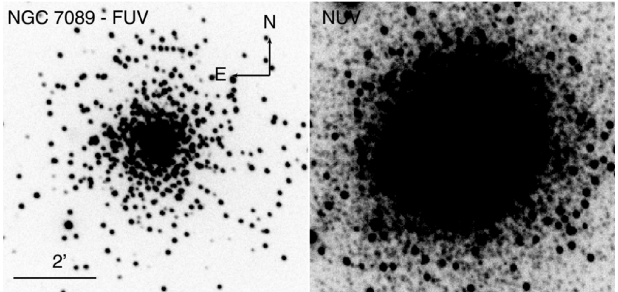
Figure 6. from Ultraviolet Properties of Galactic Globular Clusters with GALEX. I. The Color-Magnitude Diagrams Schiavon et al. 2012 AJ 143 121 doi:10.1088/0004-6256/143/5/121 https://dx.doi.org/10.1088/0004-6256/143/5/121 © 2012. The American Astronomical Society. All rights reserved.
