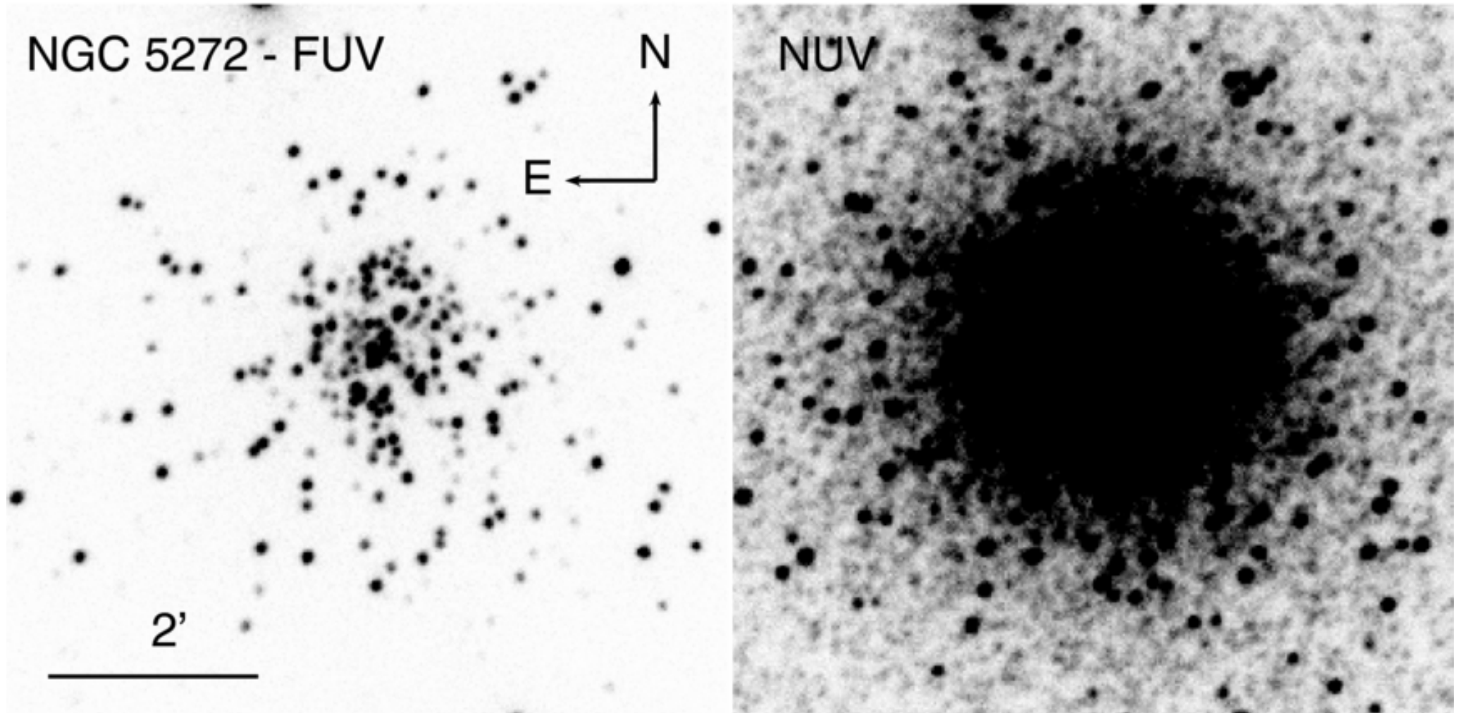
Figure 5. from Ultraviolet Properties of Galactic Globular Clusters with GALEX. I. The Color-Magnitude Diagrams Schiavon et al. 2012 AJ 143 121 doi:10.1088/0004-6256/143/5/121 https://dx.doi.org/10.1088/0004-6256/143/5/121 © 2012. The American Astronomical Society. All rights reserved.
