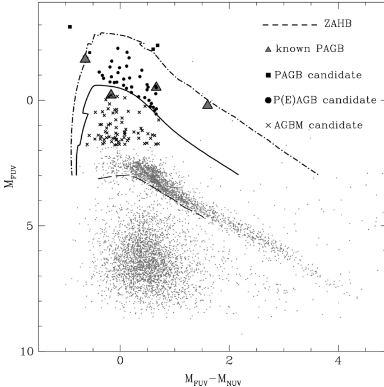
Figure 15. from Ultraviolet Properties of Galactic Globular Clusters with GALEX. I. The Color-Magnitude Diagrams Schiavon et al. 2012 AJ 143 121 doi:10.1088/0004-6256/143/5/121 https://dx.doi.org/10.1088/0004-6256/143/5/121 © 2012. The American Astronomical Society. All rights reserved.
