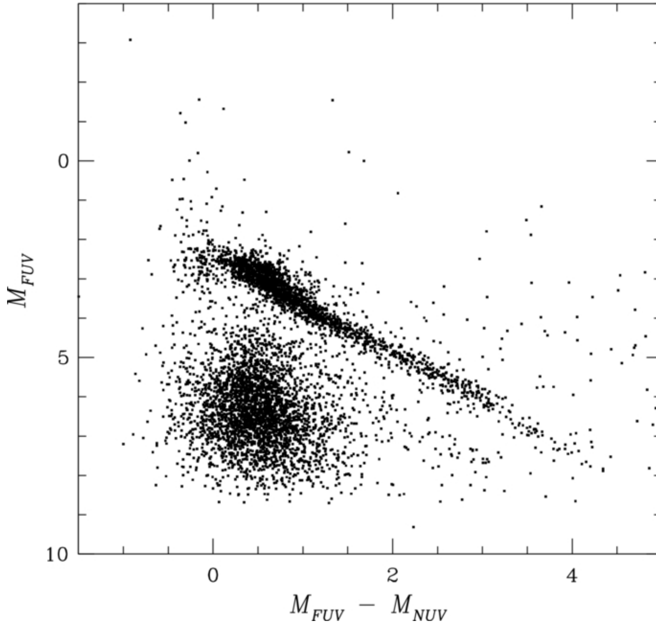
Figure 14. from Ultraviolet Properties of Galactic Globular Clusters with GALEX. I. The Color-Magnitude Diagrams Schiavon et al. 2012 AJ 143 121 doi:10.1088/0004-6256/143/5/121 https://dx.doi.org/10.1088/0004-6256/143/5/121 © 2012. The American Astronomical Society. All rights reserved.
