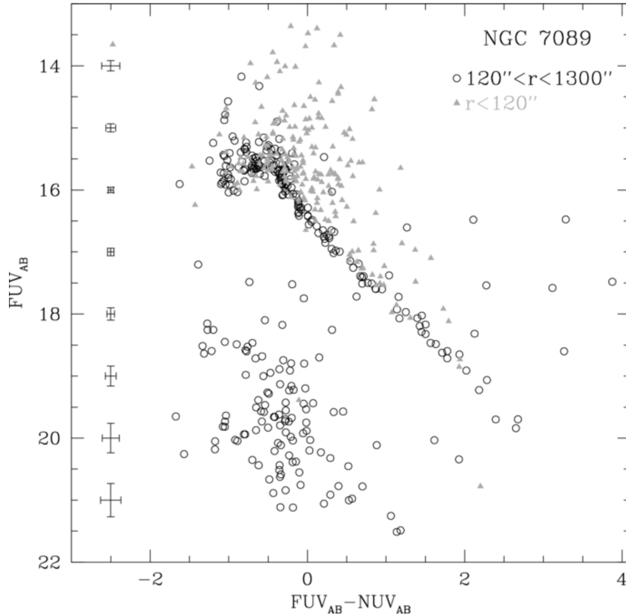
Figure 13. from Ultraviolet Properties of Galactic Globular Clusters with GALEX. I. The Color-Magnitude Diagrams Schiavon et al. 2012 AJ 143 121 doi:10.1088/0004-6256/143/5/121 https://dx.doi.org/10.1088/0004-6256/143/5/121 © 2012. The American Astronomical Society. All rights reserved.
