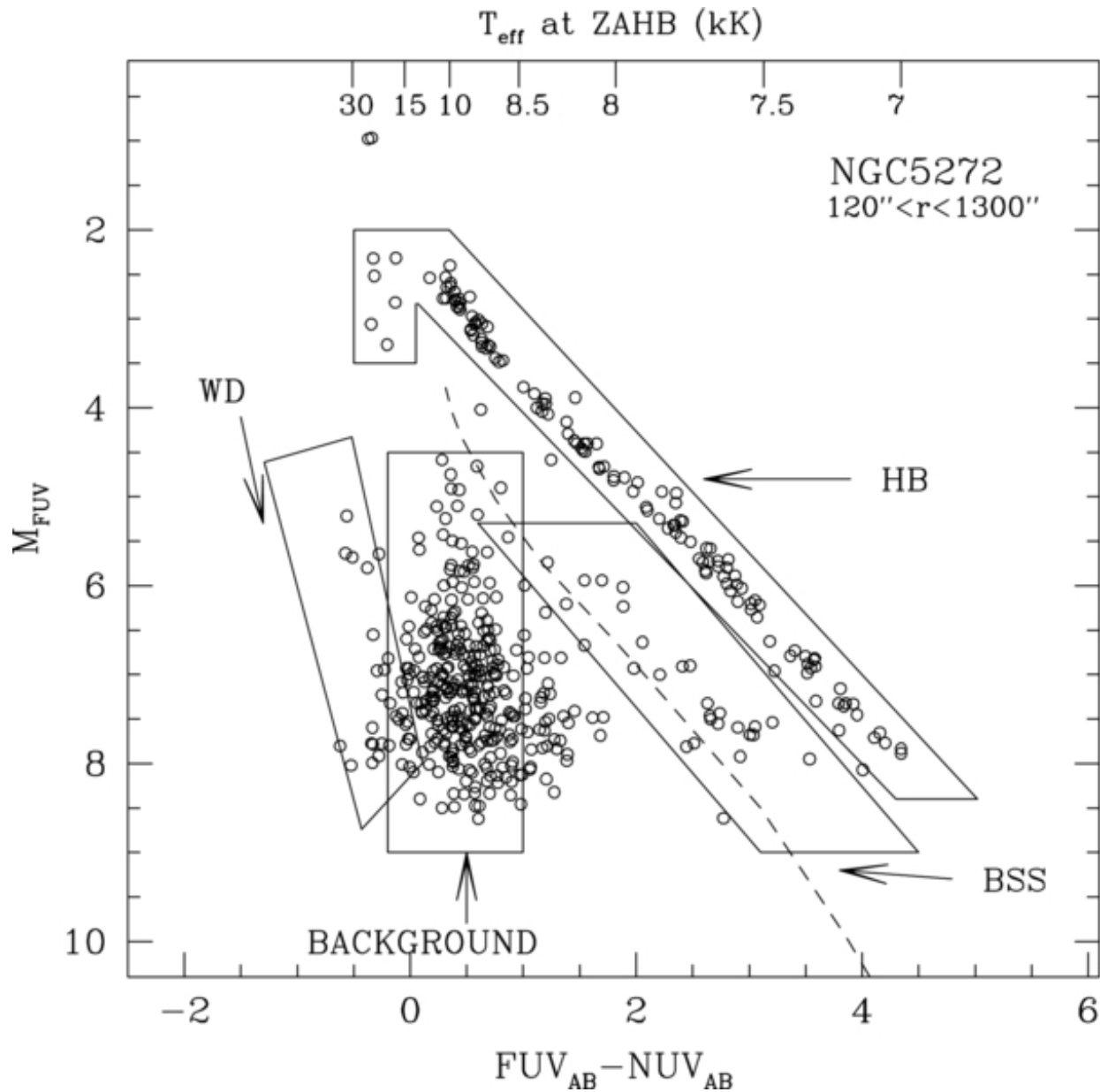
Figure 12. from Ultraviolet Properties of Galactic Globular Clusters with GALEX. I. The Color-Magnitude Diagrams Schiavon et al. 2012 AJ 143 121 doi:10.1088/0004-6256/143/5/121 https://dx.doi.org/10.1088/0004-6256/143/5/121 © 2012. The American Astronomical Society. All rights reserved.
