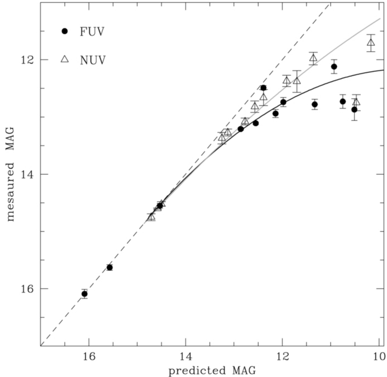
Figure 10. from Ultraviolet Properties of Galactic Globular Clusters with GALEX. I. The Color-Magnitude Diagrams Schiavon et al. 2012 AJ 143 121 doi:10.1088/0004-6256/143/5/121 https://dx.doi.org/10.1088/0004-6256/143/5/121 © 2012. The American Astronomical Society. All rights reserved.
