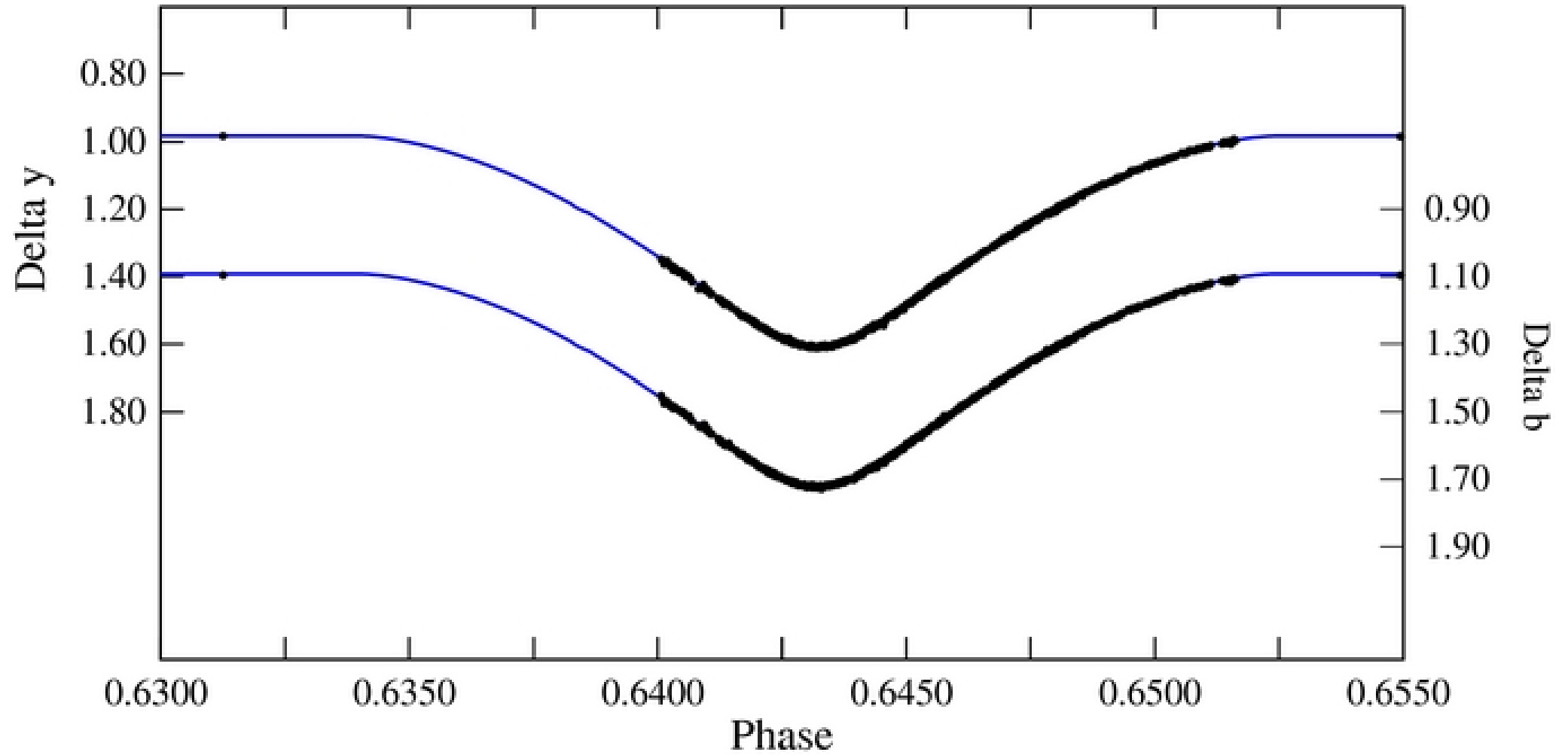
Figure 5. from Absolute Properties of the Highly Eccentric, Solar-type Eclipsing Binary HD 74057 Sowell, Henry, & Fekel 2012 AJ 143 5 doi:10.1088/0004-6256/143/1/5 https://dx.doi.org/10.1088/0004-6256/143/1/5 © 2012. The American Astronomical Society. All rights reserved.
