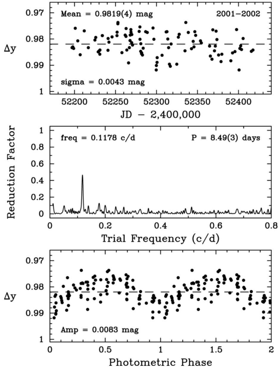
Figure 1. from Absolute Properties of the Highly Eccentric, Solar-type Eclipsing Binary HD 74057 Sowell, Henry, & Fekel 2012 AJ 143 5 doi:10.1088/0004-6256/143/1/5 https://dx.doi.org/10.1088/0004-6256/143/1/5
