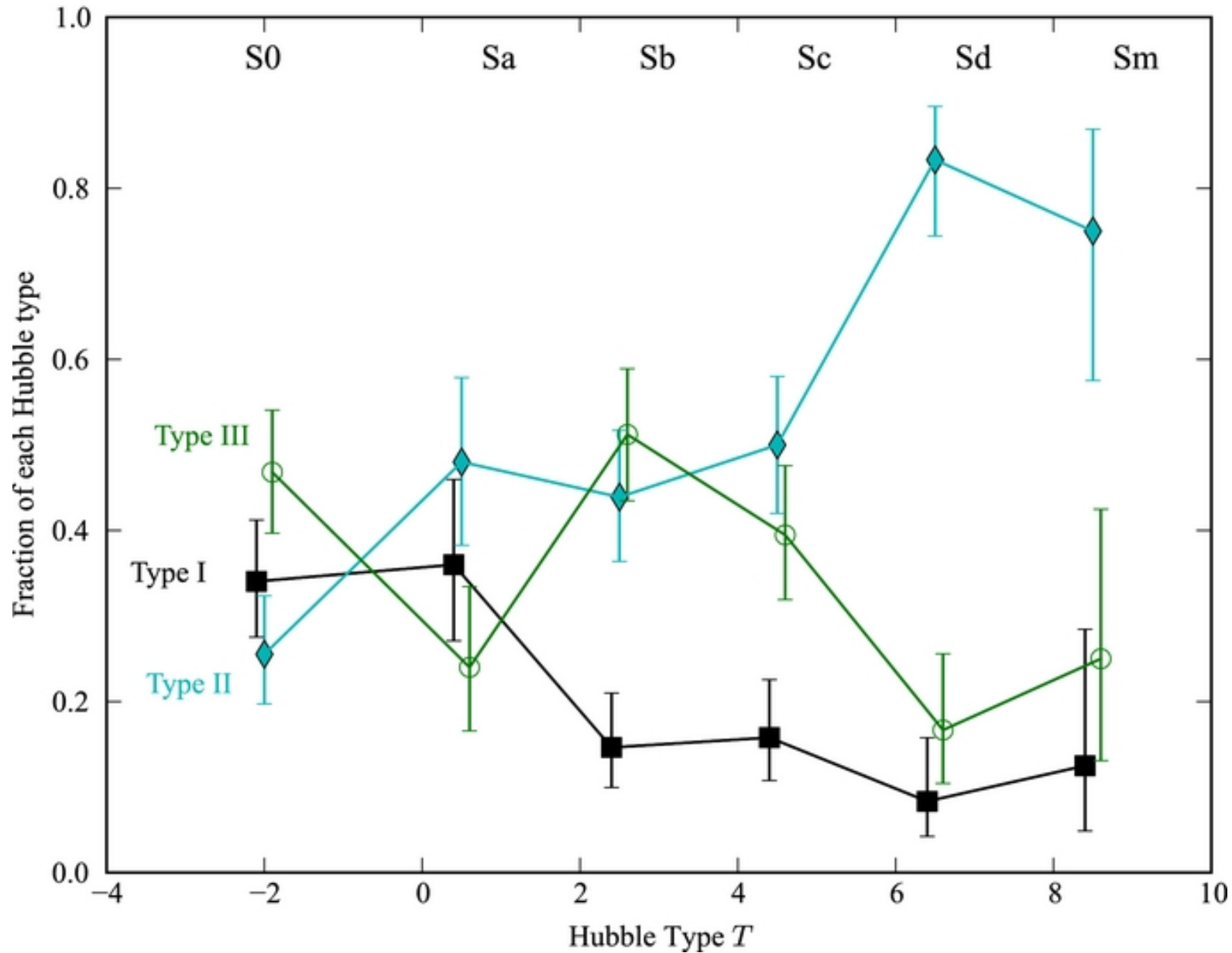
Figure 9. from The Outer Disks of Early-type Galaxies. II. Surface-brightness Profiles of Unbarred Galaxies and Trends with Hubble Type Gutiérrez et al. 2011 AJ 142 145 doi:10.1088/0004-6256/142/5/145 https://dx.doi.org/10.1088/0004-6256/142/5/145 © 2011. The American Astronomical Society. All rights reserved.
