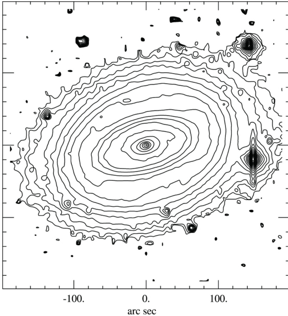
Figure 8. from The Outer Disks of Early-type Galaxies. II. Surface-brightness Profiles of Unbarred Galaxies and Trends with Hubble Type Gutiérrez et al. 2011 AJ 142 145 doi:10.1088/0004-6256/142/5/145 https://dx.doi.org/10.1088/0004-6256/142/5/145 © 2011. The American Astronomical Society. All rights reserved.
