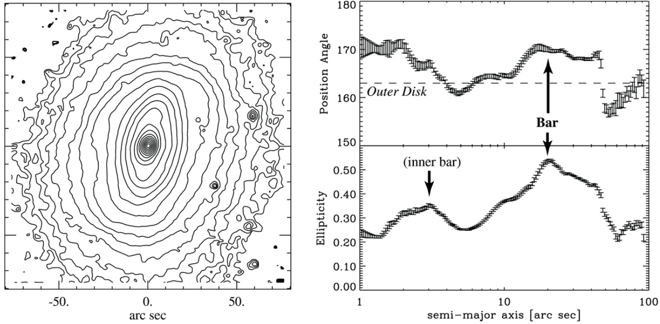
Figure 5. from The Outer Disks of Early-type Galaxies. II. Surface-brightness Profiles of Unbarred Galaxies and Trends with Hubble Type Gutiérrez et al. 2011 AJ 142 145 doi:10.1088/0004-6256/142/5/145 https://dx.doi.org/10.1088/0004-6256/142/5/145 © 2011. The American Astronomical Society. All rights reserved.
