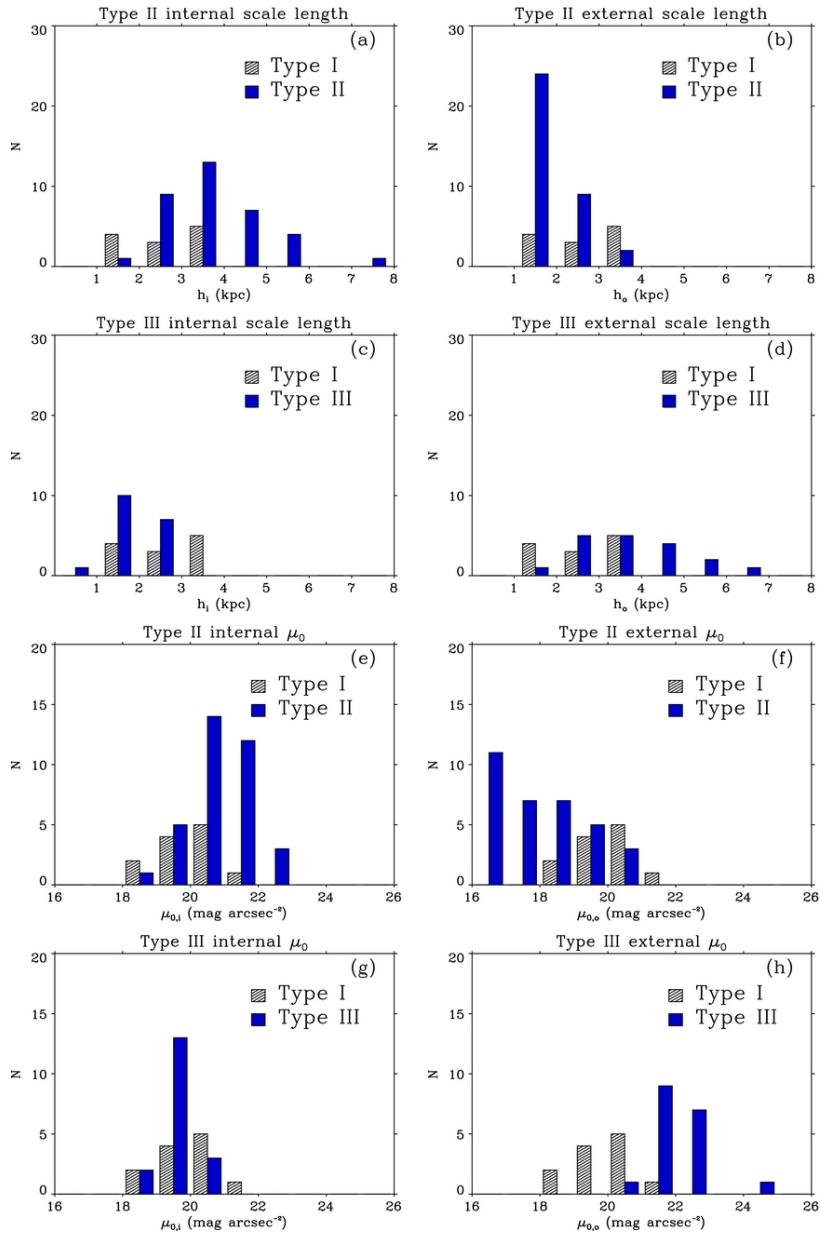
Figure 12. from The Outer Disks of Early-type Galaxies. II. Surface-brightness Profiles of Unbarred Galaxies and Trends with Hubble Type Gutiérrez et al. 2011 AJ 142 145 doi:10.1088/0004-6256/142/5/145 https://dx.doi.org/10.1088/0004-6256/142/5/145
