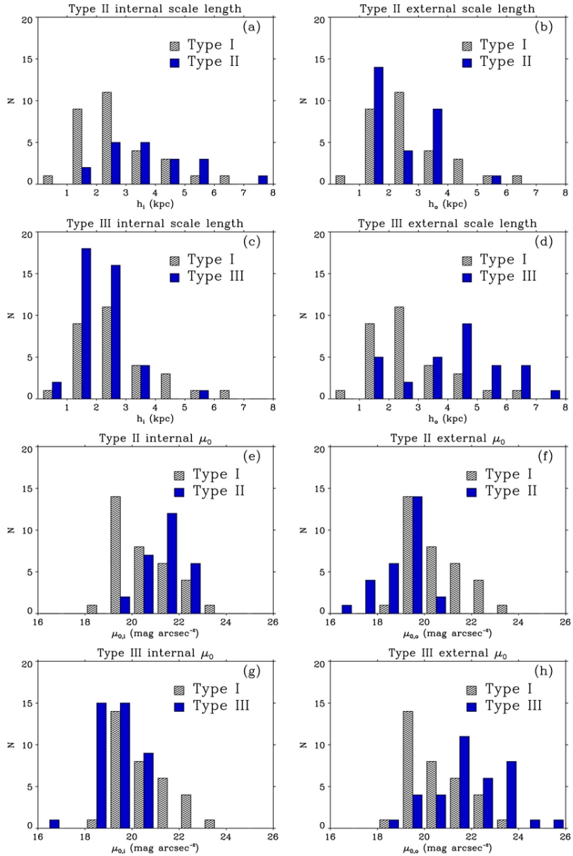
Figure 11. from The Outer Disks of Early-type Galaxies. II. Surface-brightness Profiles of Unbarred Galaxies and Trends with Hubble Type Gutiérrez et al. 2011 AJ 142 145 doi:10.1088/0004-6256/142/5/145 https://dx.doi.org/10.1088/0004-6256/142/5/145
