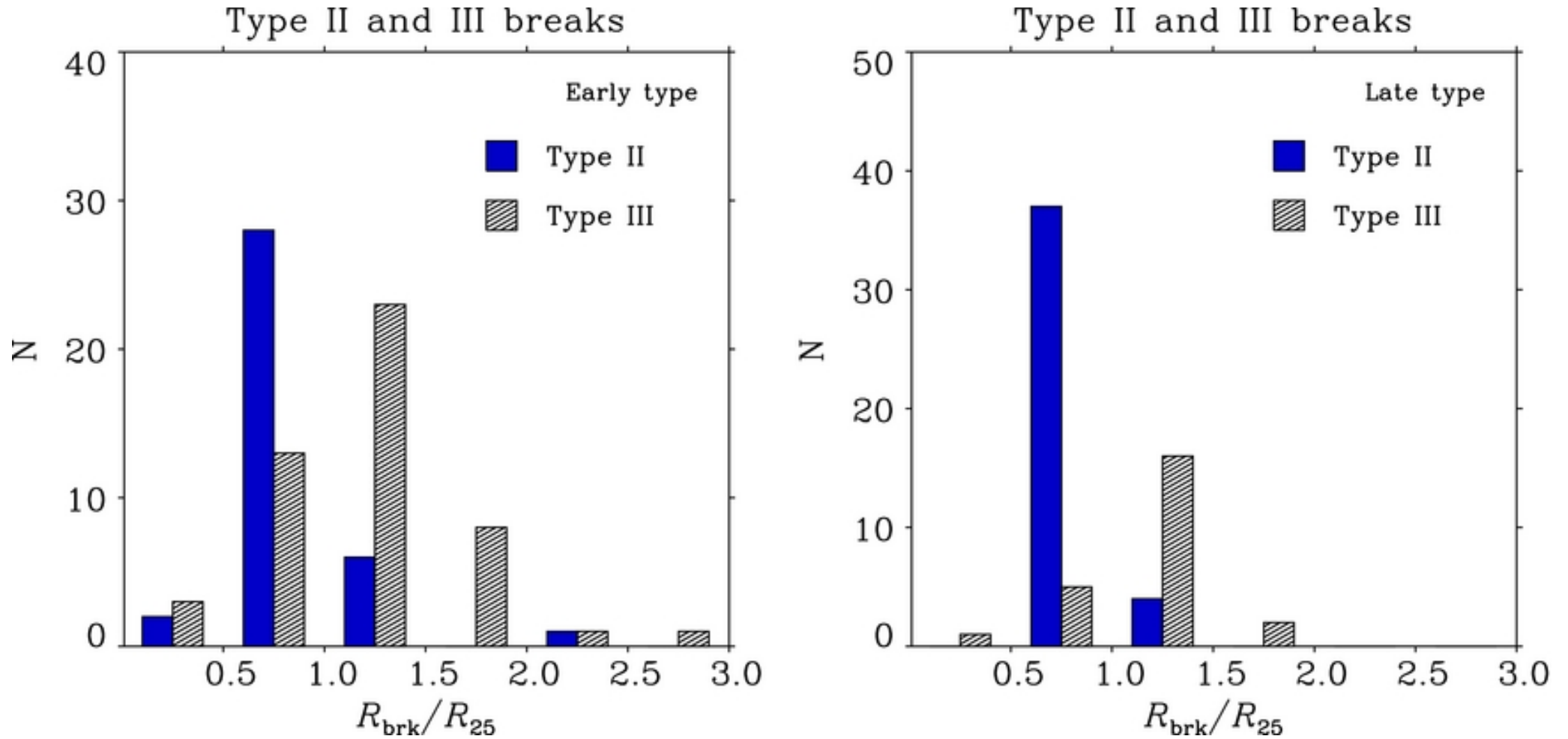
Figure 10. from The Outer Disks of Early-type Galaxies. II. Surface-brightness Profiles of Unbarred Galaxies and Trends with Hubble Type Gutiérrez et al. 2011 AJ 142 145 doi:10.1088/0004-6256/142/5/145 https://dx.doi.org/10.1088/0004-6256/142/5/145 © 2011. The American Astronomical Society. All rights reserved.
