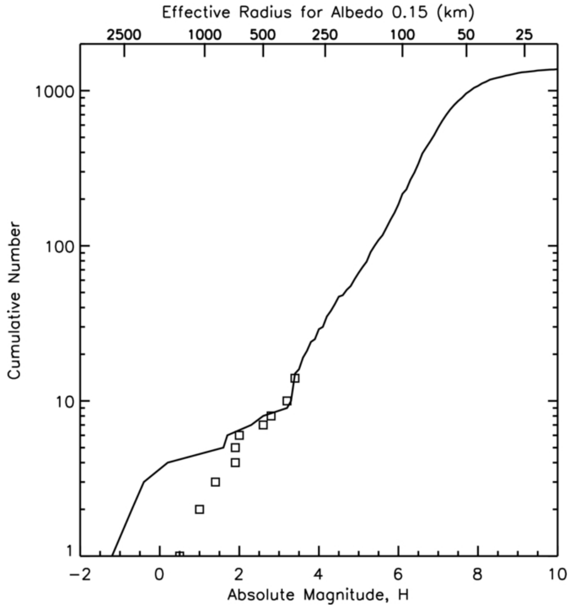
Figure 8. from A Southern Sky and Galactic Plane Survey for Bright Kuiper Belt Objects Sheppard et al. 2011 AJ 142 98 doi:10.1088/0004-6256/142/4/98 https://dx.doi.org/10.1088/0004-6256/142/4/98 © 2011. The American Astronomical Society. All rights reserved.
