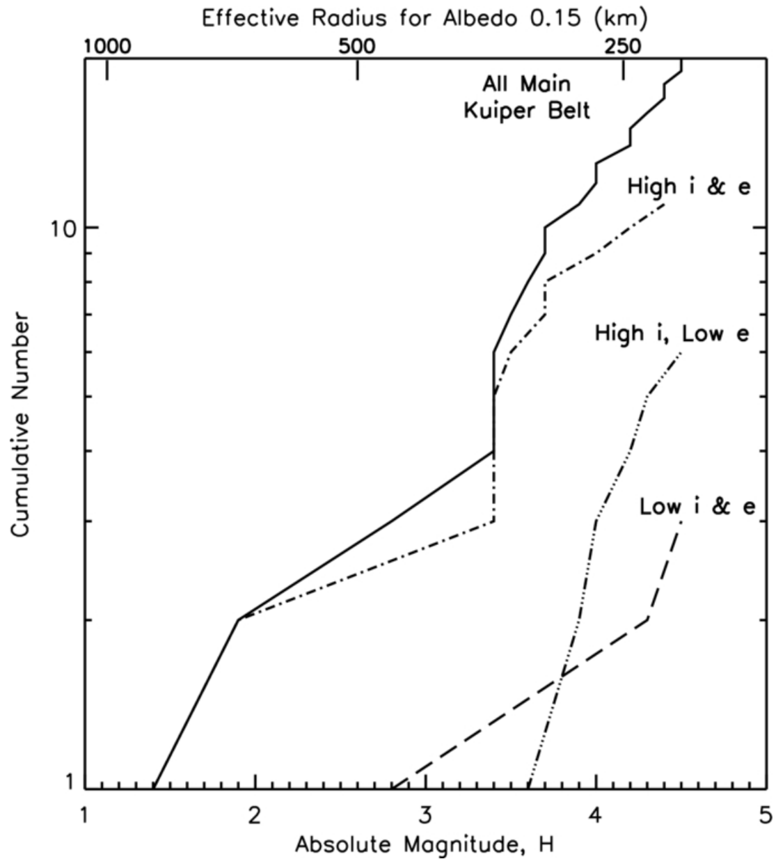
Figure 12. from A Southern Sky and Galactic Plane Survey for Bright Kuiper Belt Objects Sheppard et al. 2011 AJ 142 98 doi:10.1088/0004-6256/142/4/98 https://dx.doi.org/10.1088/0004-6256/142/4/98 © 2011. The American Astronomical Society. All rights reserved.
