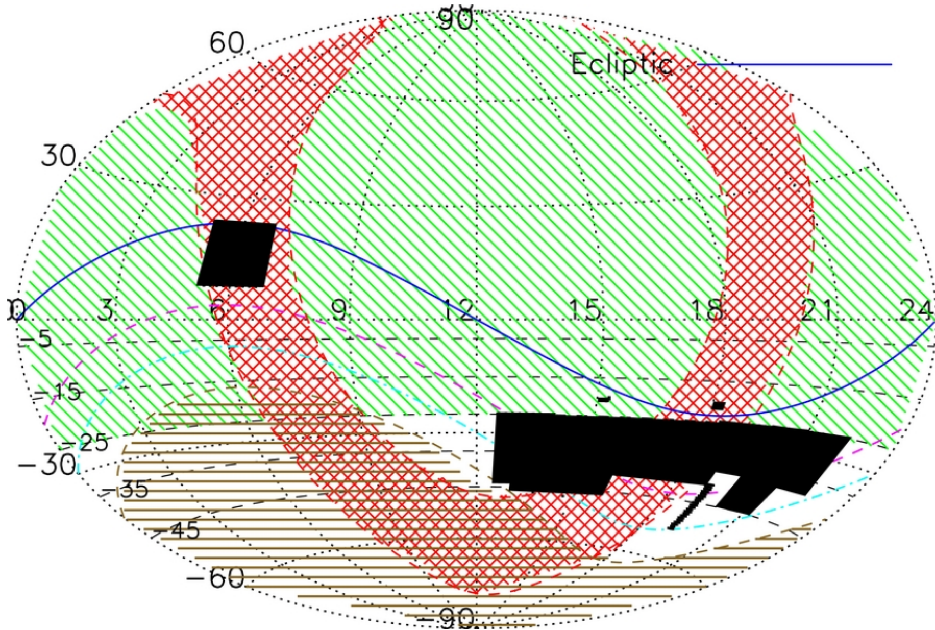
Figure 1. from A Southern Sky and Galactic Plane Survey for Bright Kuiper Belt Objects Sheppard et al. 2011 AJ 142 98 doi:10.1088/0004-6256/142/4/98 https://dx.doi.org/10.1088/0004-6256/142/4/98 © 2011. The American Astronomical Society. All rights reserved.
