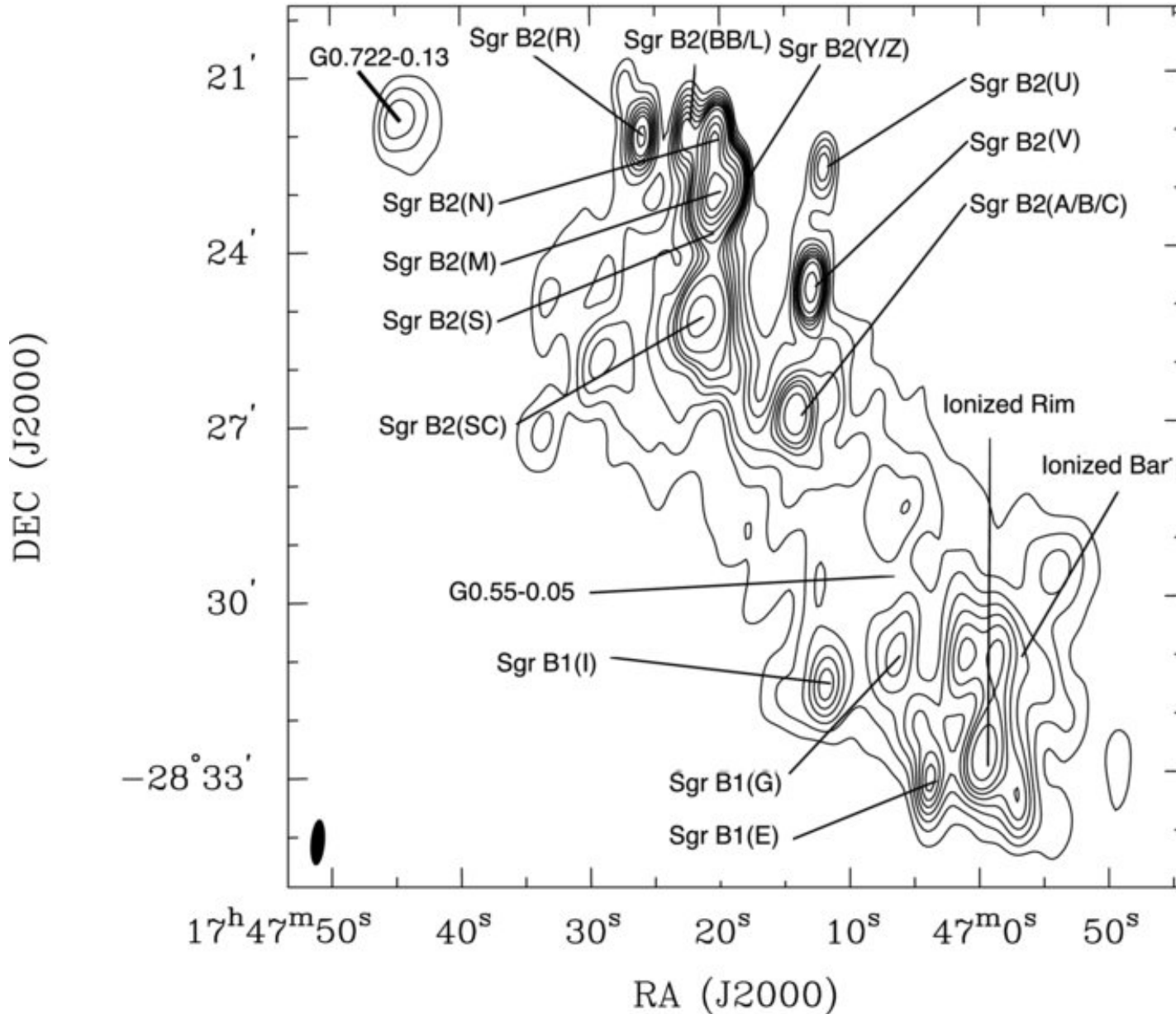
Figure 1. from Australia Telescope Compact Array Radio Continuum 1384 and 2368 MHz Observations of Sagittarius B Jones et al. 2011 AJ 141 82 doi:10.1088/0004-6256/141/3/82 https://dx.doi.org/10.1088/0004-6256/141/3/82 © 2011. The American Astronomical Society. All rights reserved.
