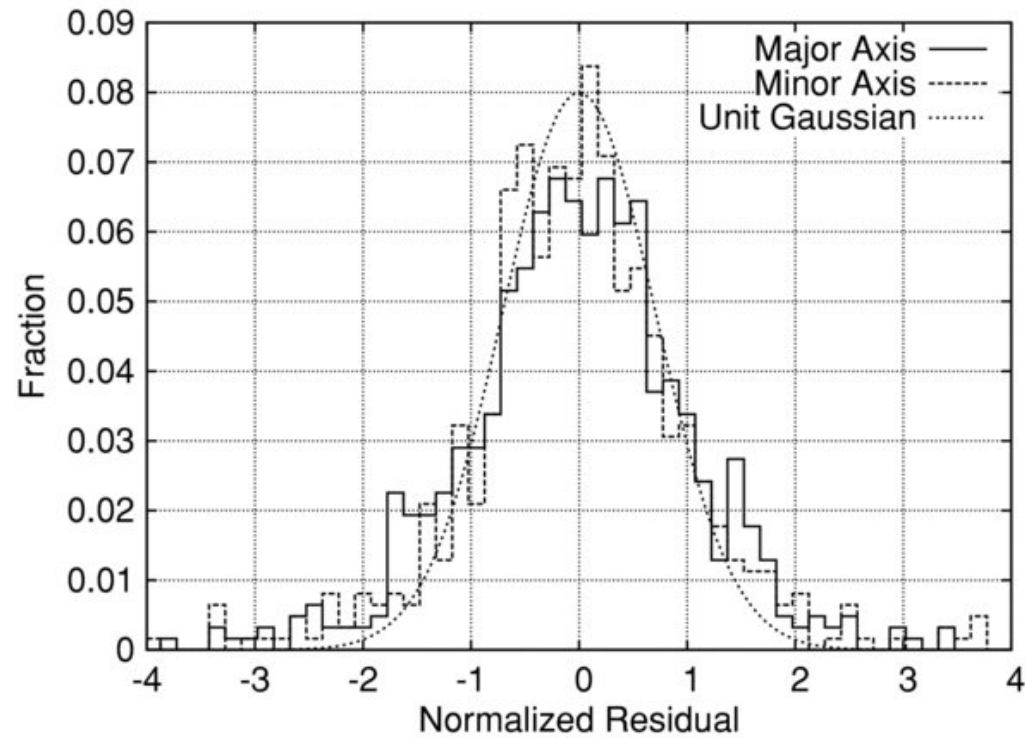
Figure 7. from The Phases Differential Astrometry Data Archive. I. Measurements and Description MUTERSPAUGH ET AL. 2010 AJ 140 1579 doi:10.1088/0004-6256/140/6/1579 https://dx.doi.org/10.1088/0004-6256/140/6/1579 © 2010. The American Astronomical Society. All rights reserved.
