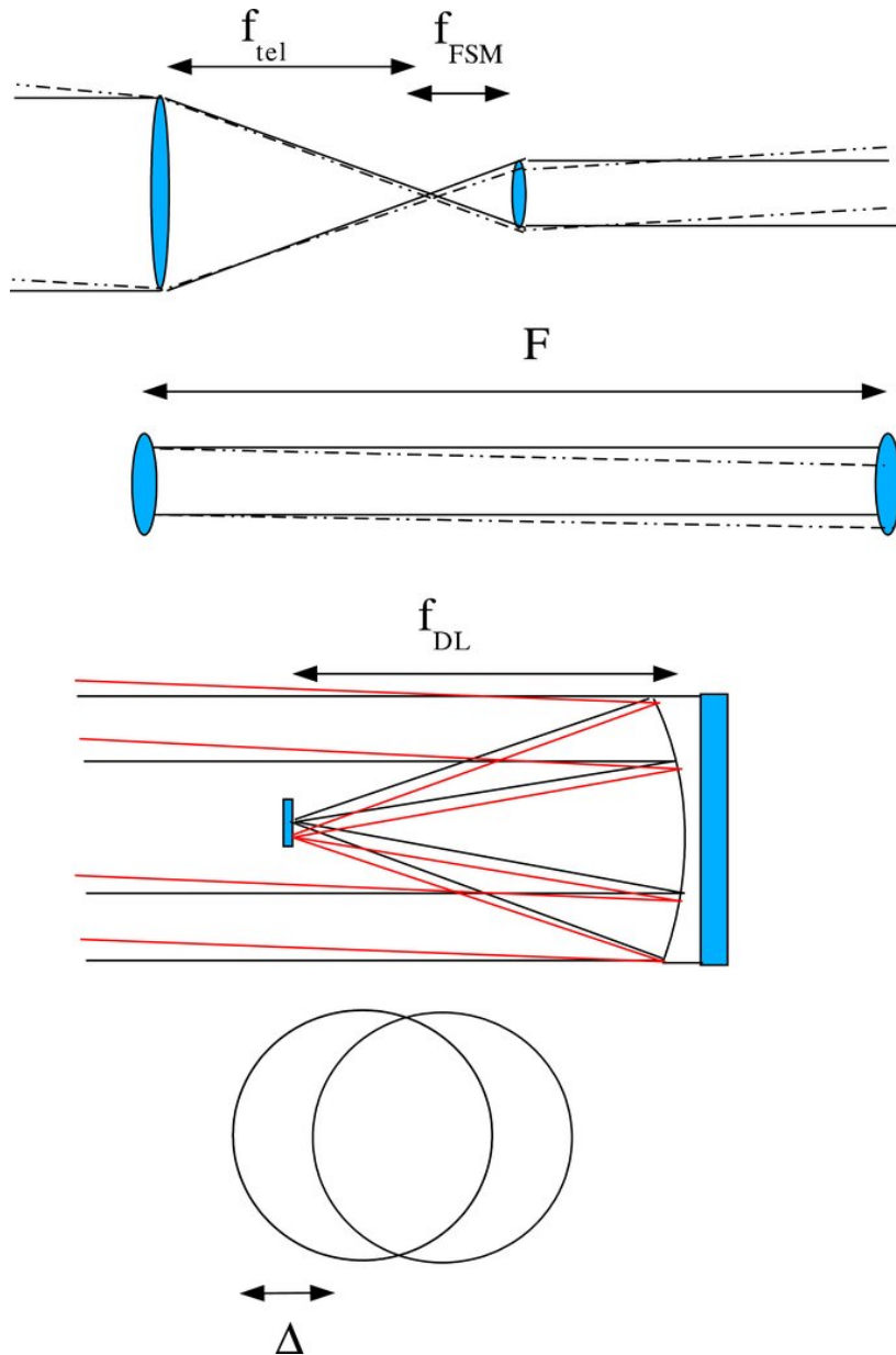
Figure 5. from The Phases Differential Astrometry Data Archive. I. Measurements and Description MUTERSPAUGH ET AL. 2010 AJ 140 1579 doi:10.1088/0004-6256/140/6/1579 https://dx.doi.org/10.1088/0004-6256/140/6/1579 © 2010. The American Astronomical Society. All rights reserved.
