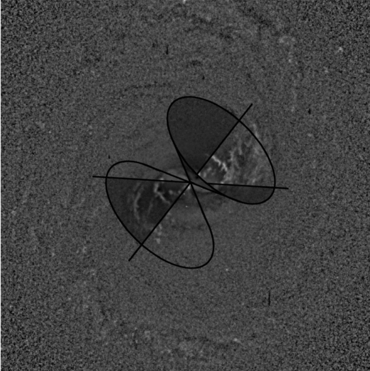
Figure 5. from Modeling the Outflow in the Narrow-line Region of Markarian 573: Biconical Illumination of a Gaseous Disk FISCHER ET AL. 2010 AJ 140 577 doi:10.1088/0004-6256/140/2/577 https://dx.doi.org/10.1088/0004-6256/140/2/577 © 2010. The American Astronomical Society. All rights reserved.
