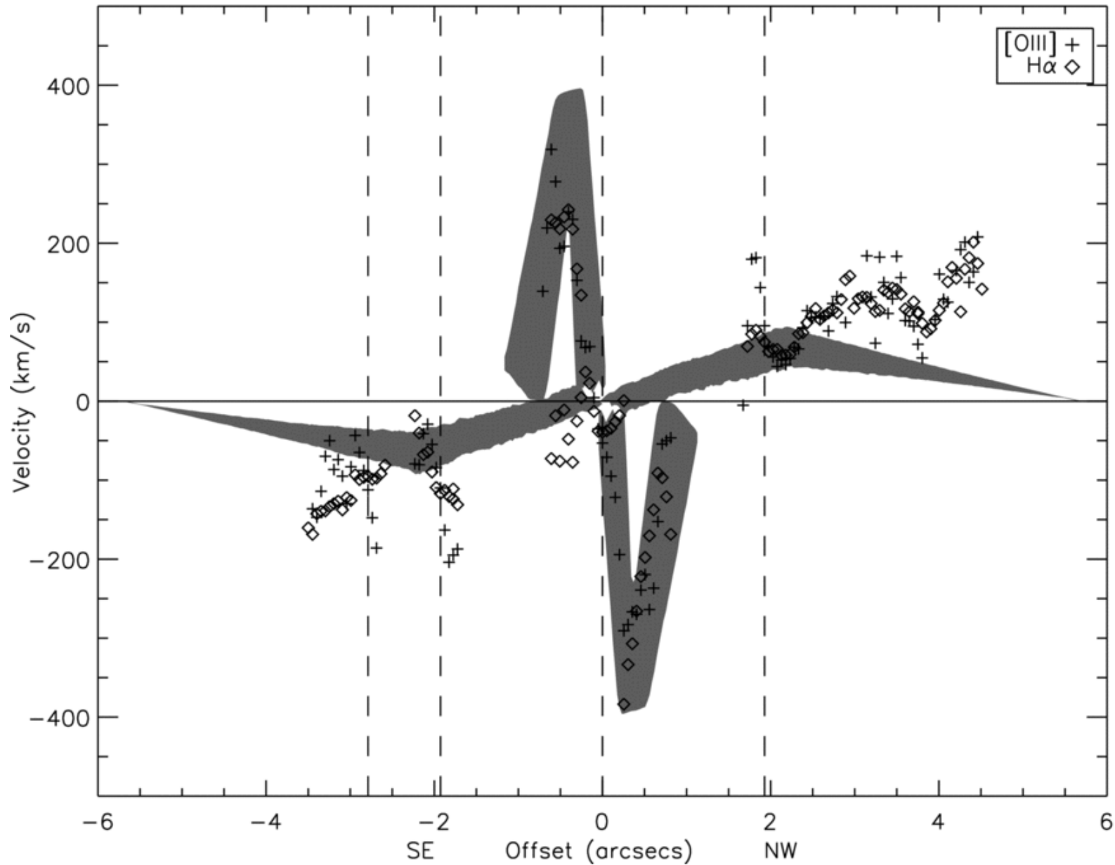
Figure 3. from Modeling the Outflow in the Narrow-line Region of Markarian 573: Biconical Illumination of a Gaseous Disk FISCHER ET AL. 2010 AJ 140 577 doi:10.1088/0004-6256/140/2/577 https://dx.doi.org/10.1088/0004-6256/140/2/577 © 2010. The American Astronomical Society. All rights reserved.
