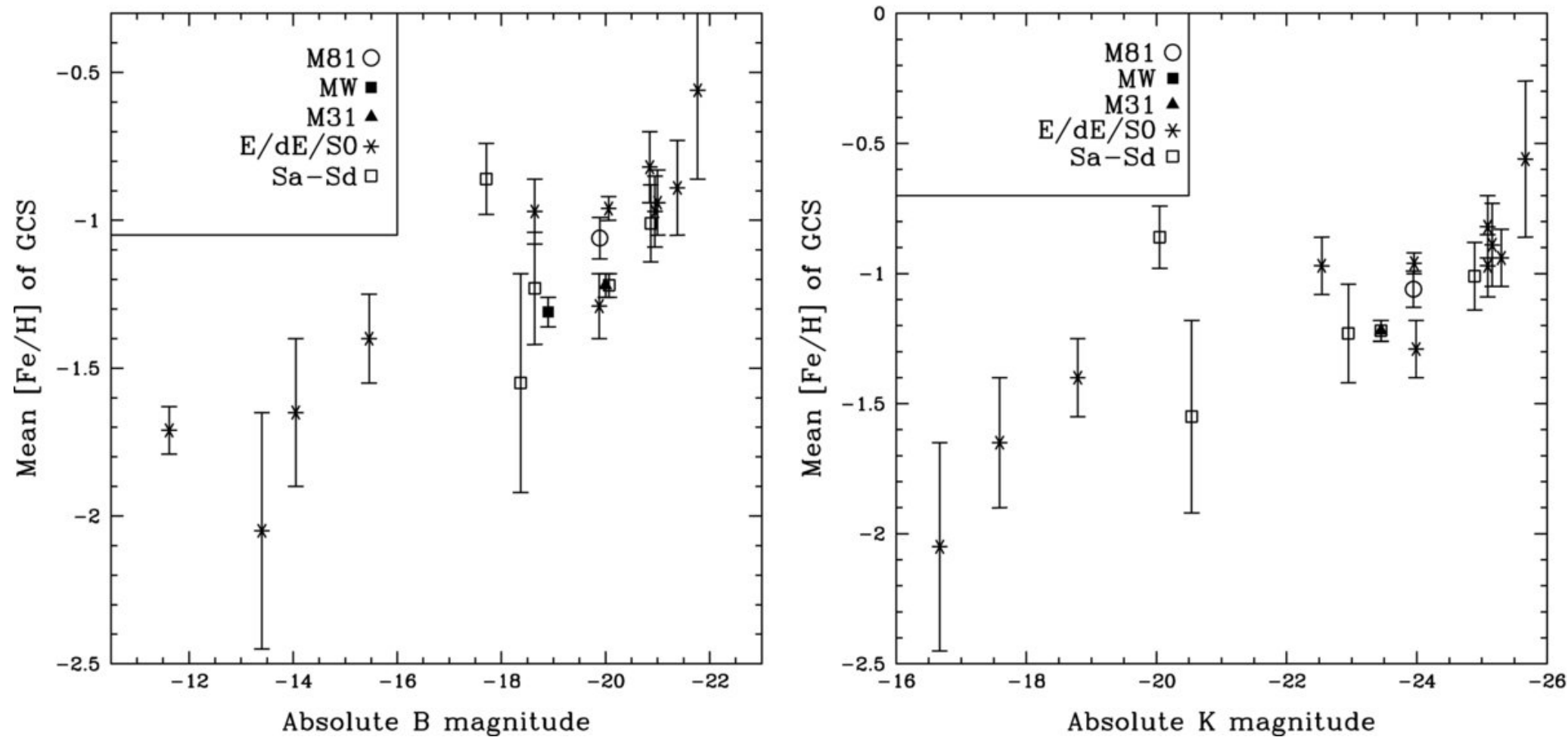
Figure 8. from Spectroscopy of M81 Globular Clusters NANTAIS & HUCHRA 2010 AJ 139 2620 doi:10.1088/0004-6256/139/6/2620 https://dx.doi.org/10.1088/0004-6256/139/6/2620 © 2010. The American Astronomical Society. All rights reserved.
