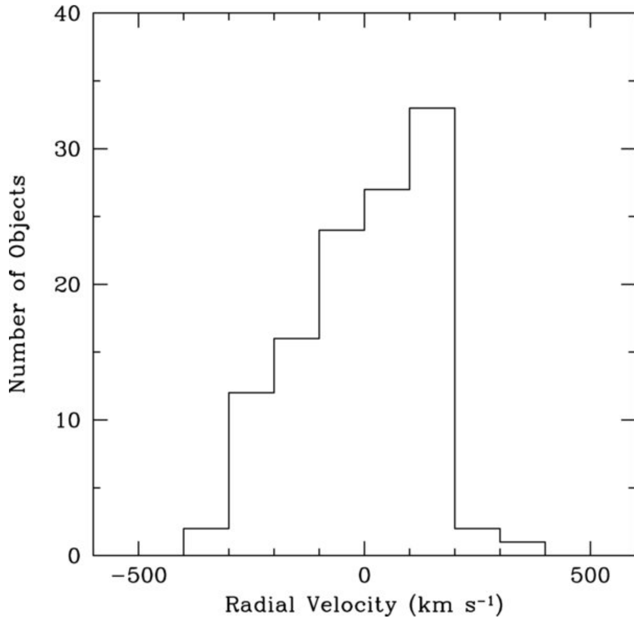
Figure 3. from Spectroscopy of M81 Globular Clusters NANTAIS & HUCHRA 2010 AJ 139 2620 doi:10.1088/0004-6256/139/6/2620 https://dx.doi.org/10.1088/0004-6256/139/6/2620 © 2010. The American Astronomical Society. All rights reserved.
