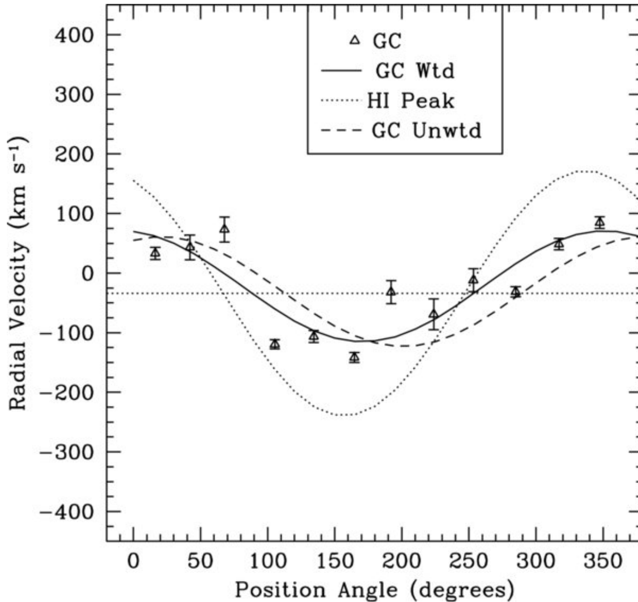
Figure 13. from Spectroscopy of M81 Globular Clusters NANTAIS & HUCHRA 2010 AJ 139 2620 doi:10.1088/0004-6256/139/6/2620 https://dx.doi.org/10.1088/0004-6256/139/6/2620 © 2010. The American Astronomical Society. All rights reserved.
